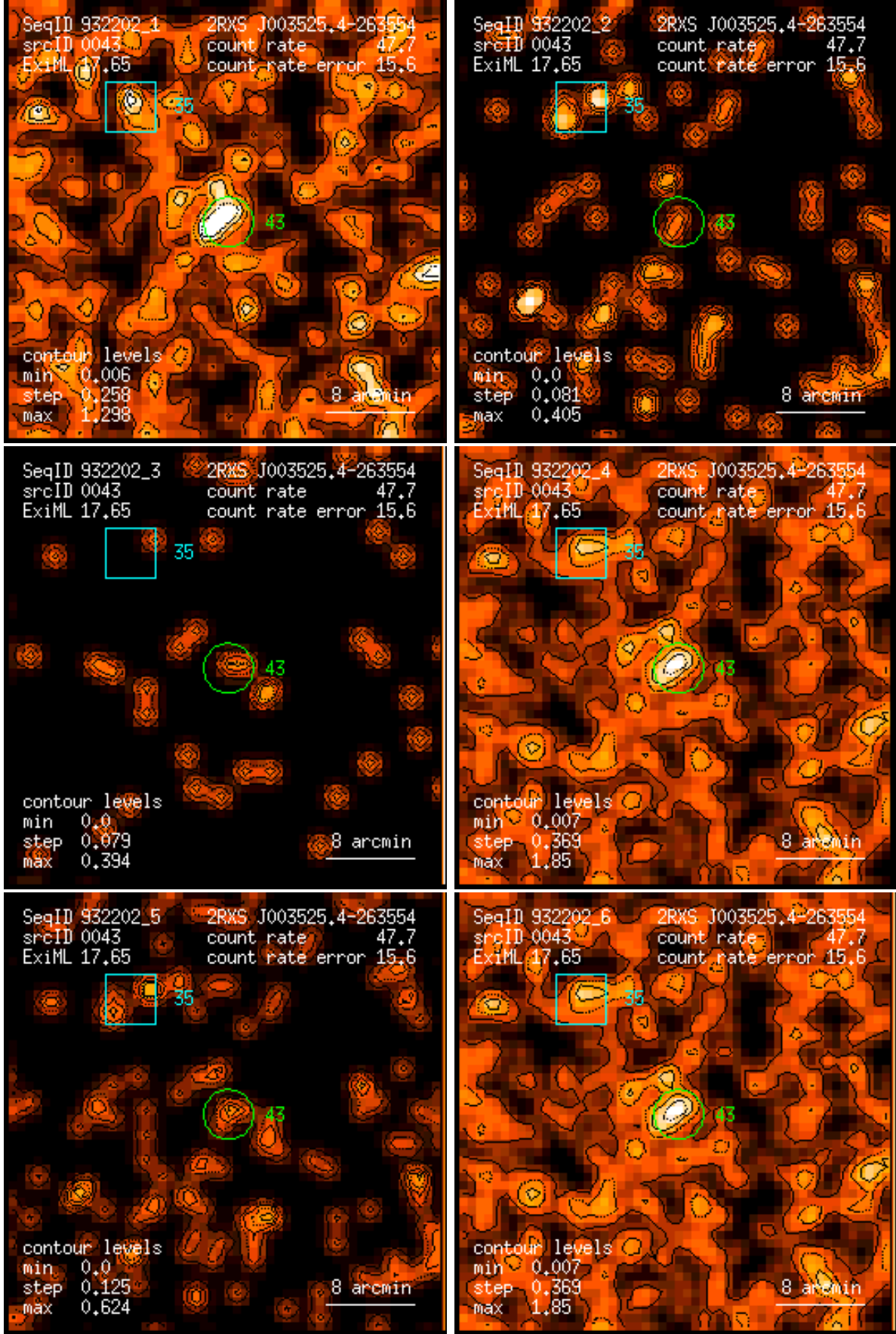
Figure 43: RASS 932202: detection 0043: band rate images, Gaussian filter: (1) PSPC channels 11 – 41, (2) 52 – 90, (3) 91 – 201, (4) 11 – 235, (5) 52 – 201, (6) 11 – 201. Broad band rates in counts/ks. Band rate contour levels in counts/ks/arcmin 2 .
