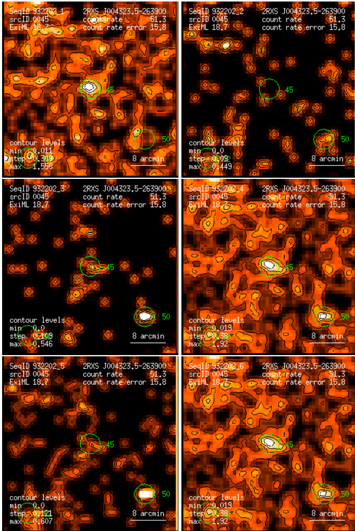
Figure 45: RASS 932202: detection 0045: band rate images, Gaussian filter: (1) PSPC channels 11 – 41, (2) 52 – 90, (3) 91 – 201, (4) 11 – 235, (5) 52 – 201, (6) 11 – 201. Broad band rates in counts/ks. Band rate contour levels in counts/ks/arcmin 2 .
