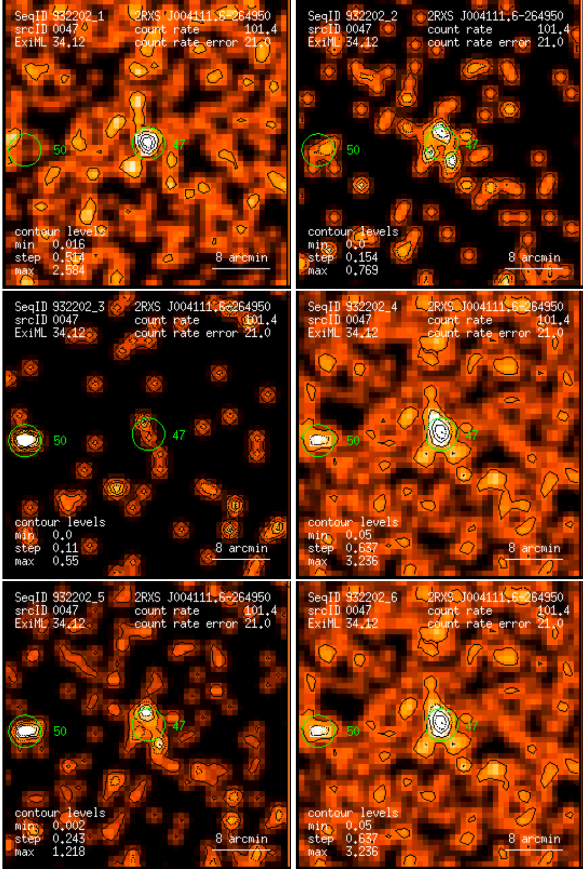
Figure 47: RASS 932202: detection 0047: band rate images, Gaussian filter: (1) PSPC channels 11 – 41, (2) 52 – 90, (3) 91 – 201, (4) 11 – 235, (5) 52 – 201, (6) 11 – 201. Broad band rates in counts/ks. Band rate contour levels in counts/ks/arcmin 2 .
