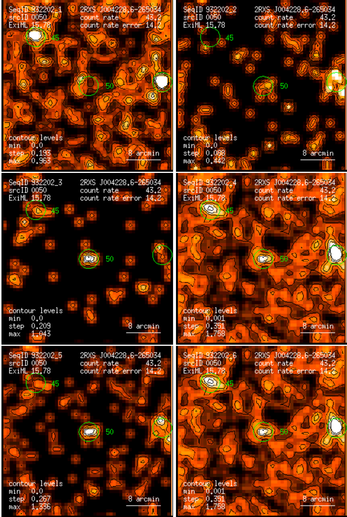
Figure 50: RASS 932202: detection 0050: band rate images, Gaussian filter: (1) PSPC channels 11 – 41, (2) 52 – 90, (3) 91 – 201, (4) 11 – 235, (5) 52 – 201, (6) 11 – 201. Broad band rates in counts/ks. Band rate contour levels in counts/ks/arcmin 2 .
