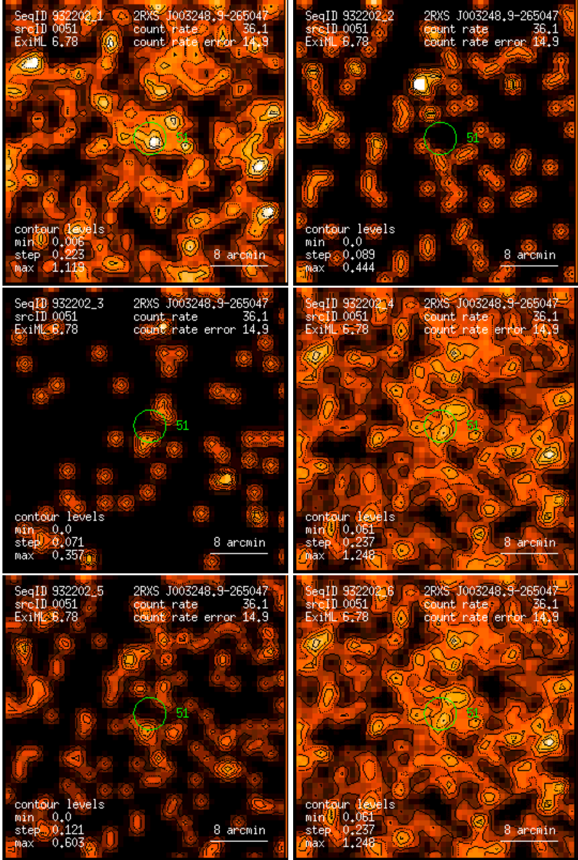
Figure 51: RASS 932202: detection 0051: band rate images, Gaussian filter: (1) PSPC channels 11 – 41, (2) 52 – 90, (3) 91 – 201, (4) 11 – 235, (5) 52 – 201, (6) 11 – 201. Broad band rates in counts/ks. Band rate contour levels in counts/ks/arcmin 2 .
