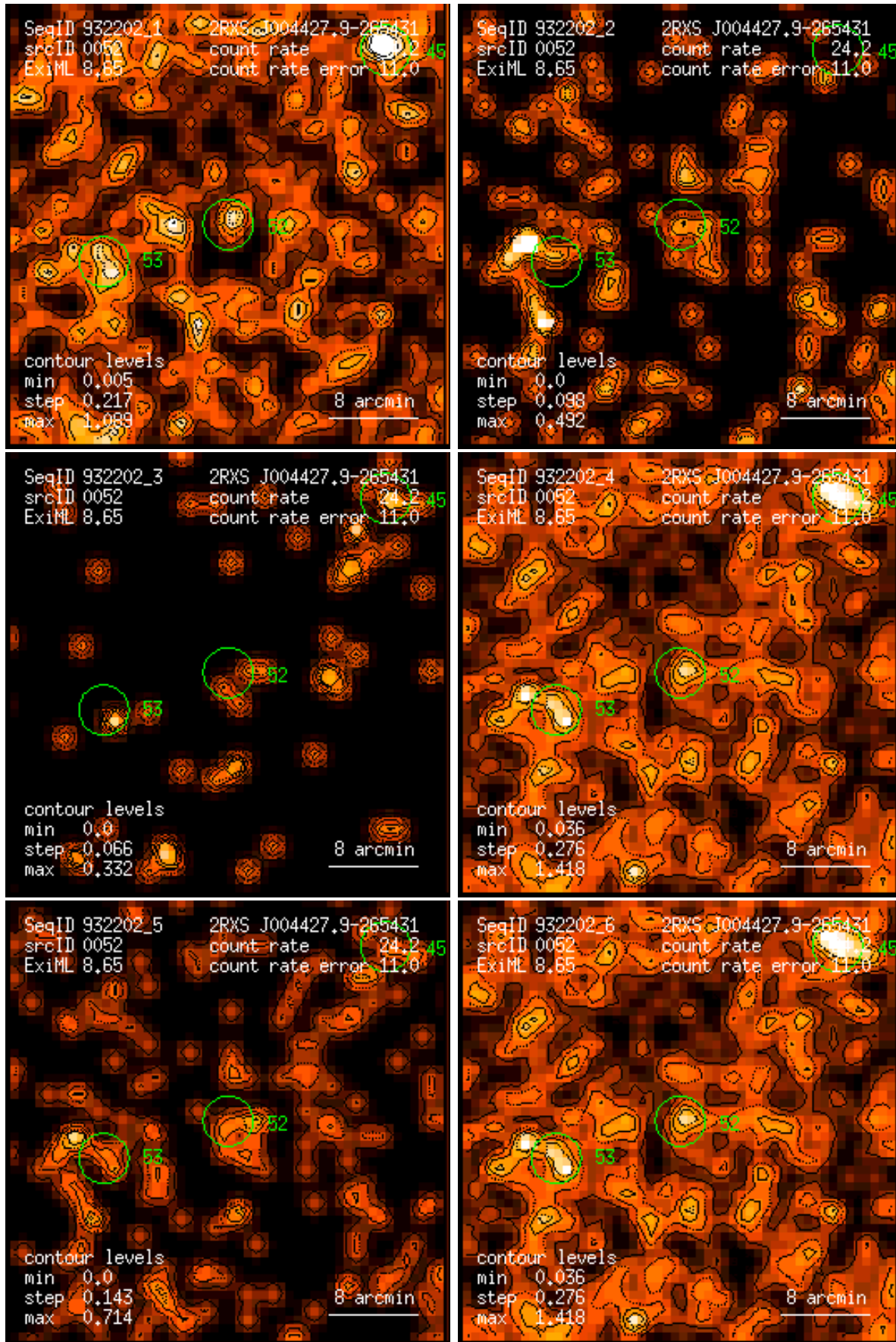
Figure 52: RASS 932202: detection 0052: band rate images, Gaussian filter: (1) PSPC channels 11 – 41, (2) 52 – 90, (3) 91 – 201, (4) 11 – 235, (5) 52 – 201, (6) 11 – 201. Broad band rates in counts/ks. Band rate contour levels in counts/ks/arcmin 2 .
