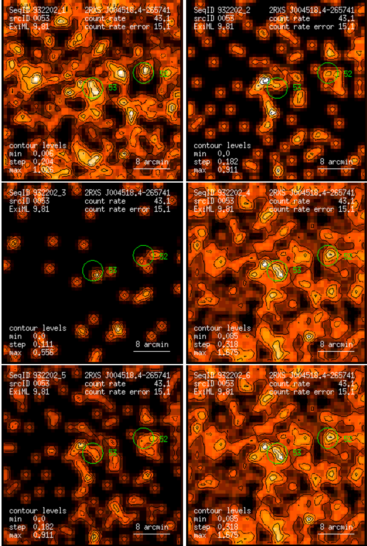
Figure 53: RASS 932202: detection 0053: band rate images, Gaussian filter: (1) PSPC channels 11 – 41, (2) 52 – 90, (3) 91 – 201, (4) 11 – 235, (5) 52 – 201, (6) 11 – 201. Broad band rates in counts/ks. Band rate contour levels in counts/ks/arcmin 2 .
