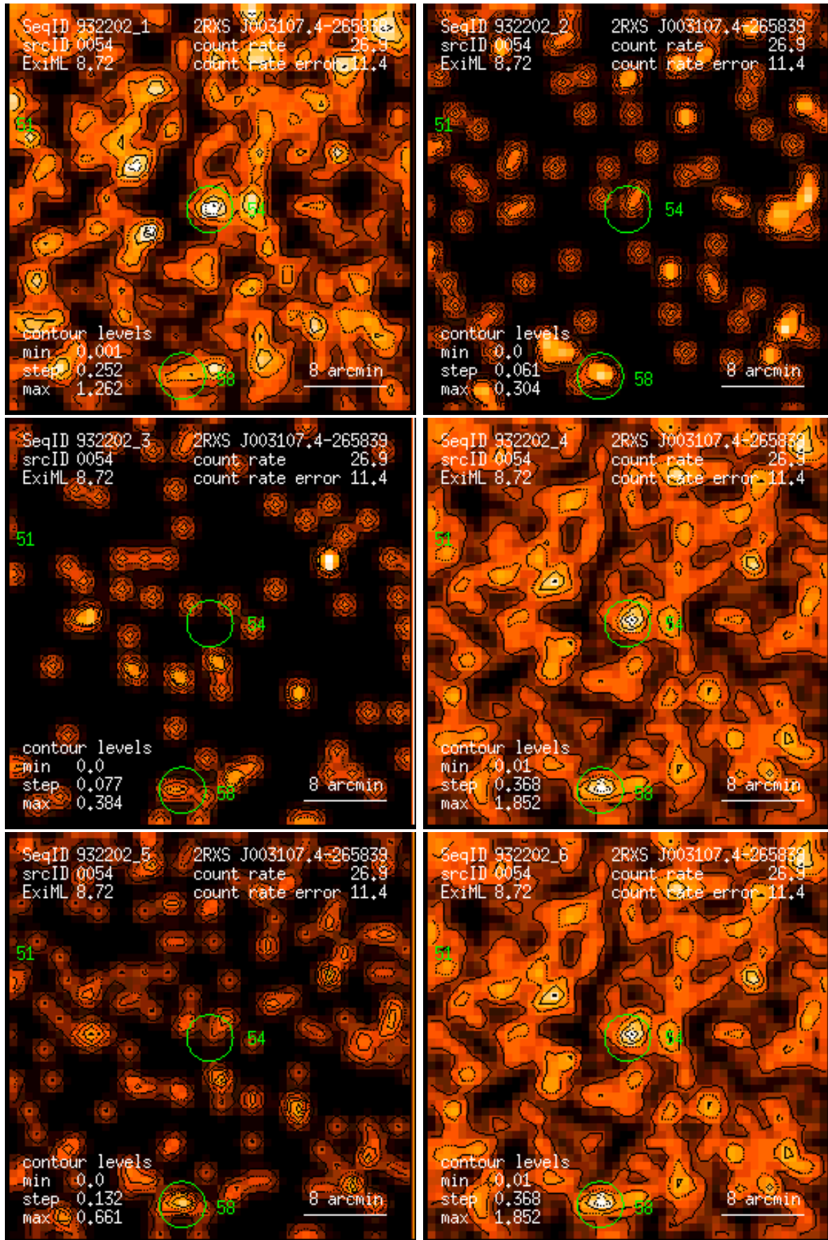
Figure 54: RASS 932202: detection 0054: band rate images, Gaussian filter: (1) PSPC channels 11 – 41, (2) 52 – 90, (3) 91 – 201, (4) 11 – 235, (5) 52 – 201, (6) 11 – 201. Broad band rates in counts/ks. Band rate contour levels in counts/ks/arcmin 2 .
