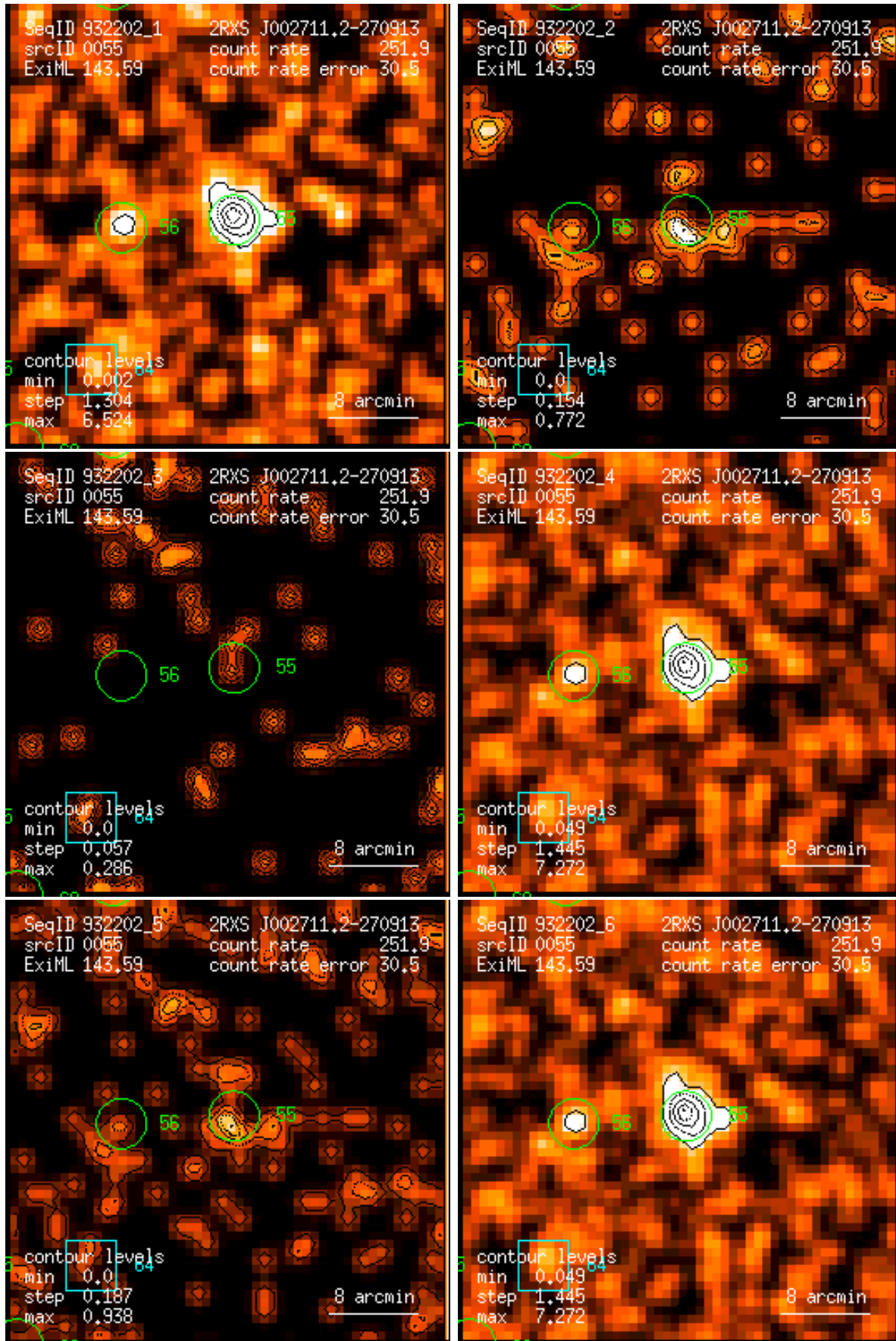
Figure 55: RASS 932202: detection 0055: band rate images, Gaussian filter: (1) PSPC channels 11 – 41, (2) 52 – 90, (3) 91 – 201, (4) 11 – 235, (5) 52 – 201, (6) 11 – 201. Broad band rates in counts/ks. Band rate contour levels in counts/ks/arcmin 2 .
