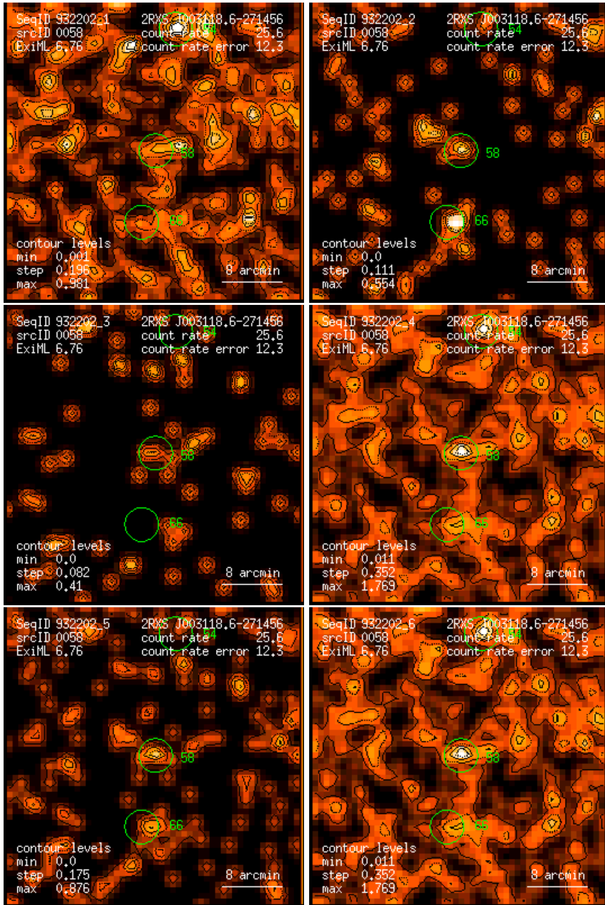
Figure 58: RASS 932202: detection 0058: band rate images, Gaussian filter: (1) PSPC channels 11 – 41, (2) 52 – 90, (3) 91 – 201, (4) 11 – 235, (5) 52 – 201, (6) 11 – 201. Broad band rates in counts/ks. Band rate contour levels in counts/ks/arcmin 2 .
