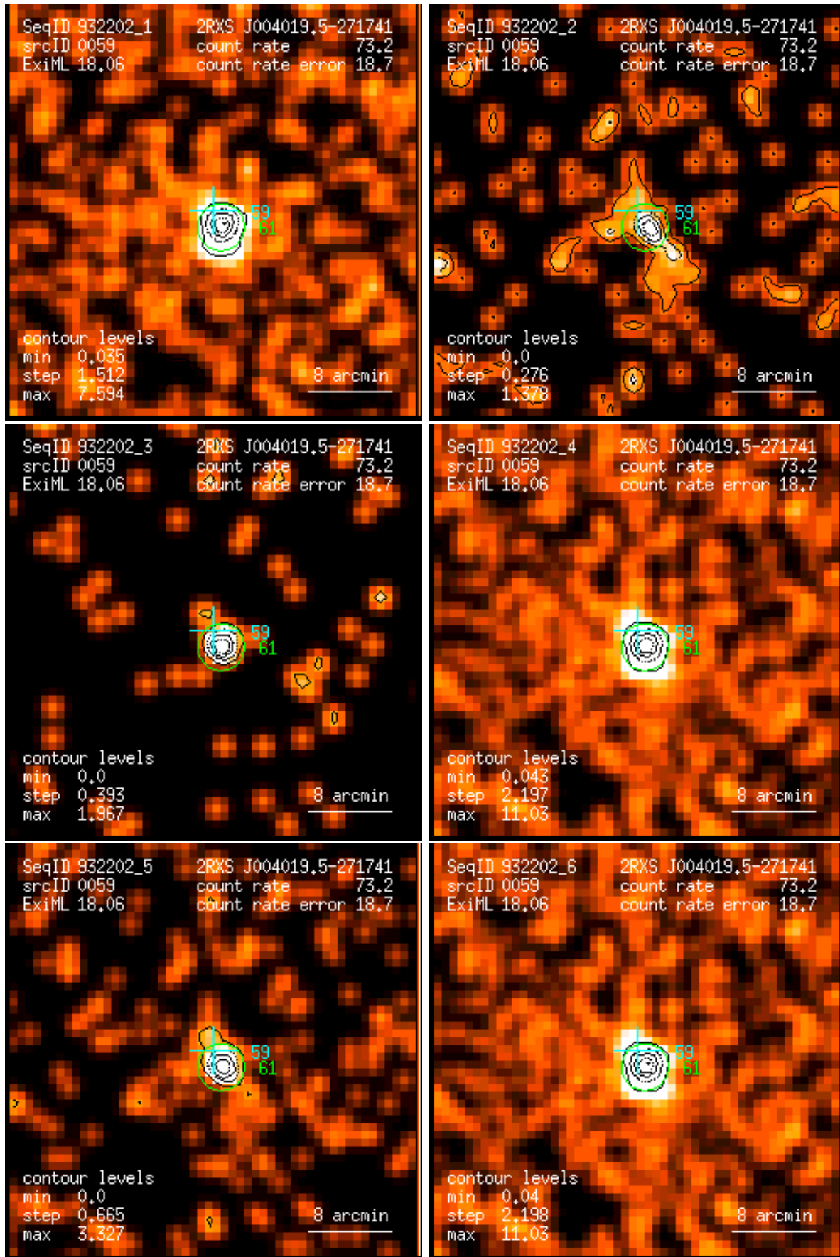
Figure 59: RASS 932202: detection 0059: band rate images, Gaussian filter: (1) PSPC channels 11 – 41, (2) 52 – 90, (3) 91 – 201, (4) 11 – 235, (5) 52 – 201, (6) 11 – 201. Broad band rates in counts/ks. Band rate contour levels in counts/ks/arcmin 2 .
