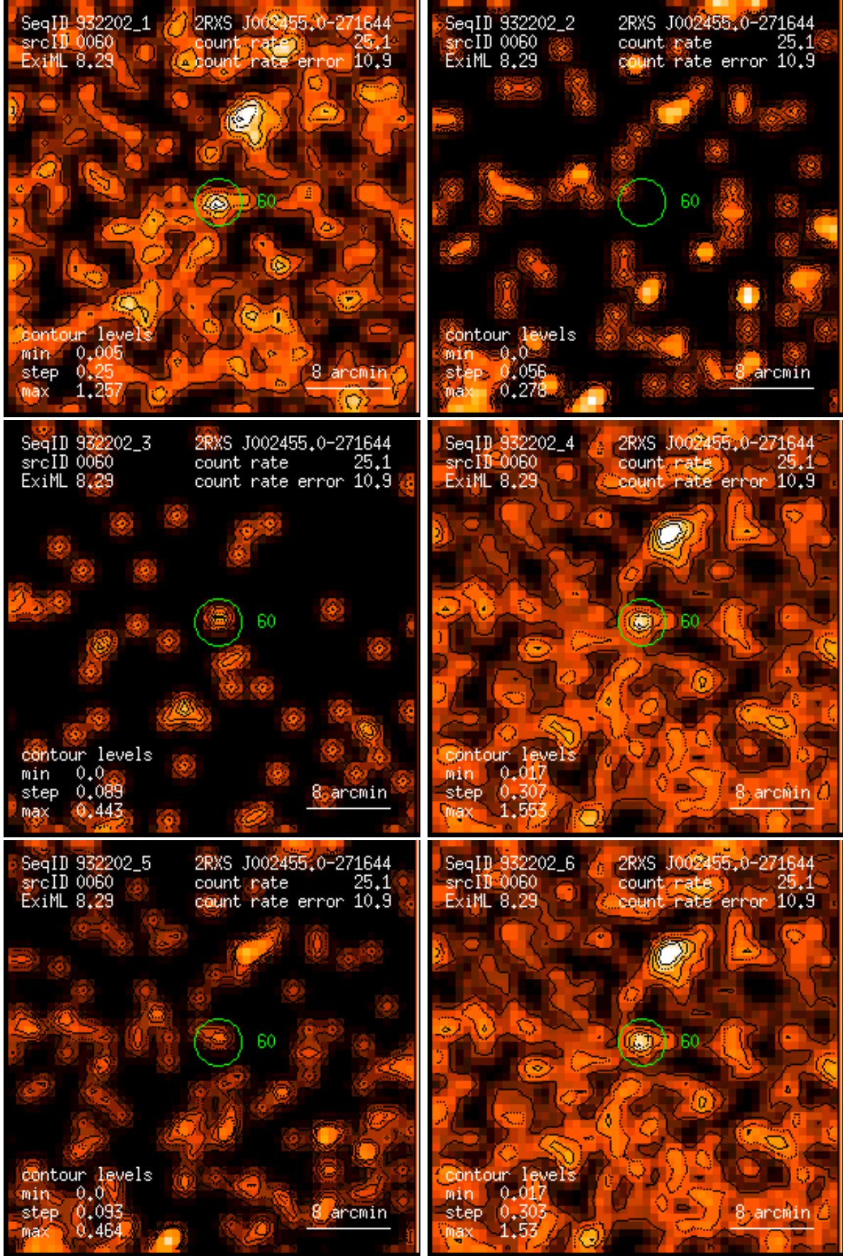
Figure 60: RASS 932202: detection 0060: band rate images, Gaussian filter: (1) PSPC channels 11 – 41, (2) 52 – 90, (3) 91 – 201, (4) 11 – 235, (5) 52 – 201, (6) 11 – 201. Broad band rates in counts/ks. Band rate contour levels in counts/ks/arcmin 2 .
