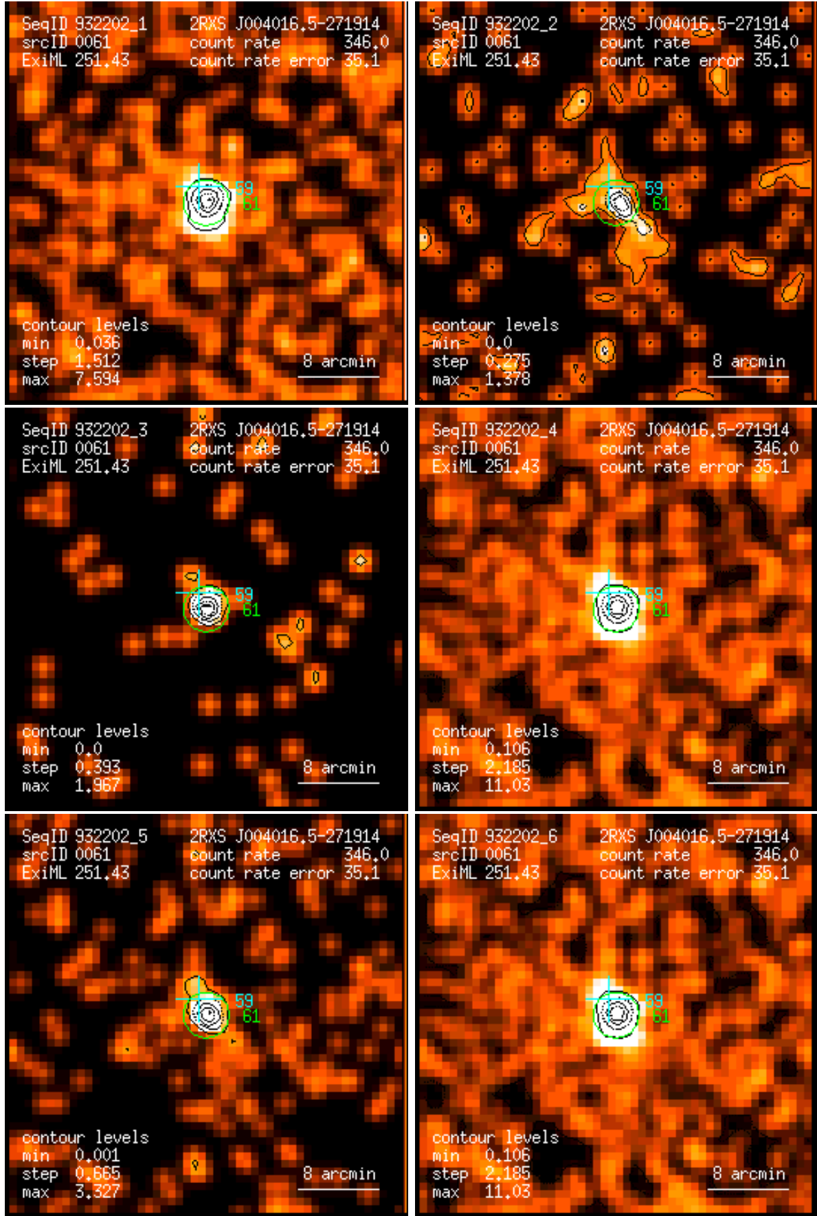
Figure 61: RASS 932202: detection 0061: band rate images, Gaussian filter: (1) PSPC channels 11 – 41, (2) 52 – 90, (3) 91 – 201, (4) 11 – 235, (5) 52 – 201, (6) 11 – 201. Broad band rates in counts/ks. Band rate contour levels in counts/ks/arcmin 2 .
