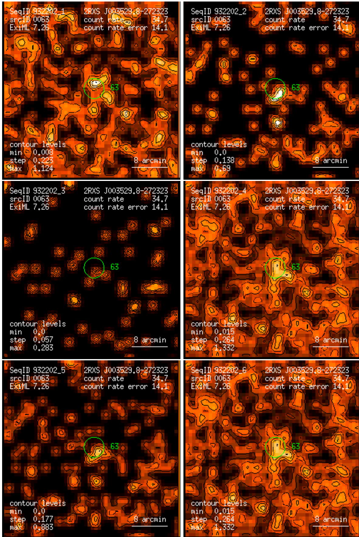
Figure 63: RASS 932202: detection 0063: band rate images, Gaussian filter: (1) PSPC channels 11 – 41, (2) 52 – 90, (3) 91 – 201, (4) 11 – 235, (5) 52 – 201, (6) 11 – 201. Broad band rates in counts/ks. Band rate contour levels in counts/ks/arcmin 2 .
