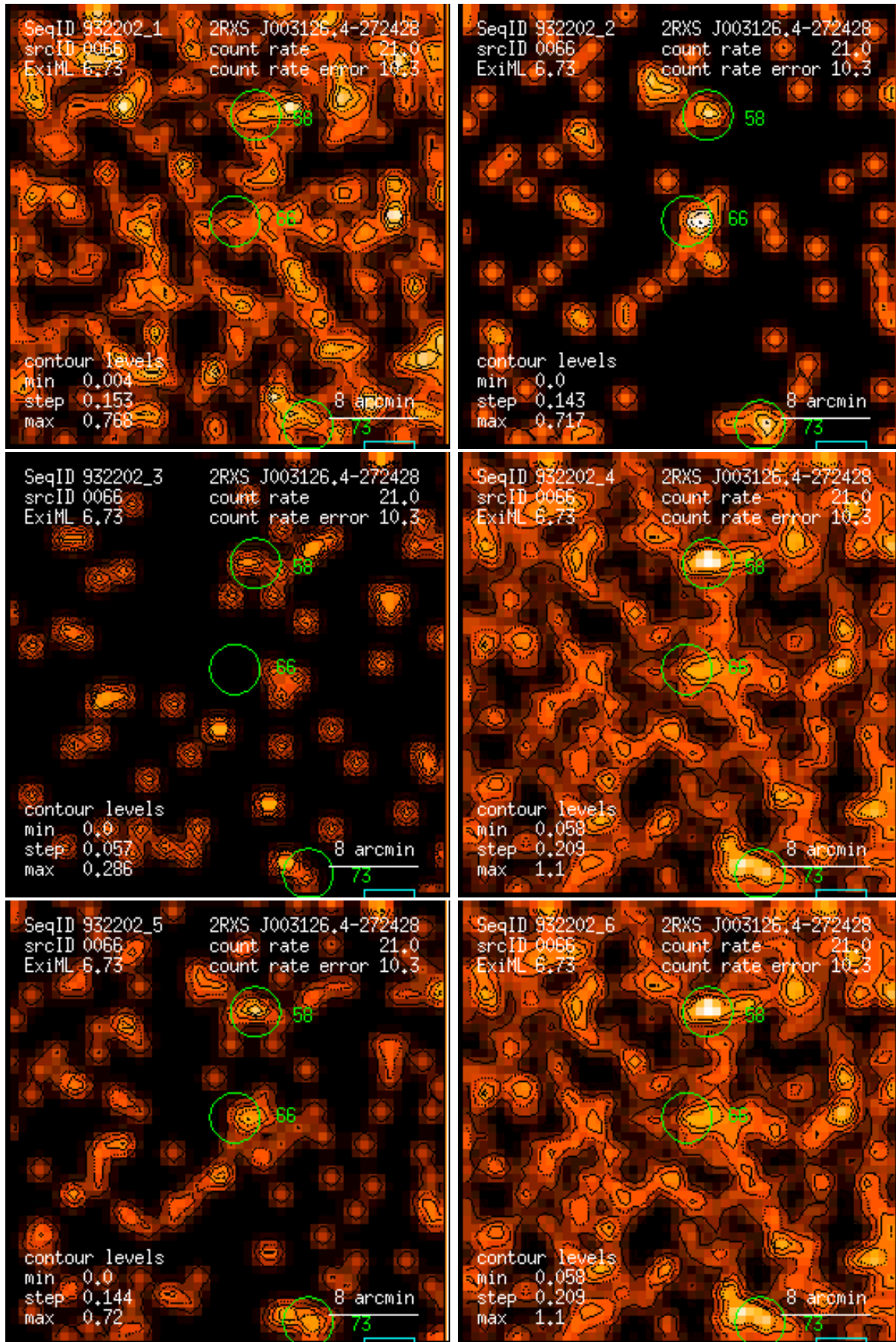
Figure 66: RASS 932202: detection 0066: band rate images, Gaussian filter: (1) PSPC channels 11 – 41, (2) 52 – 90, (3) 91 – 201, (4) 11 – 235, (5) 52 – 201, (6) 11 – 201. Broad band rates in counts/ks. Band rate contour levels in counts/ks/arcmin 2 .
