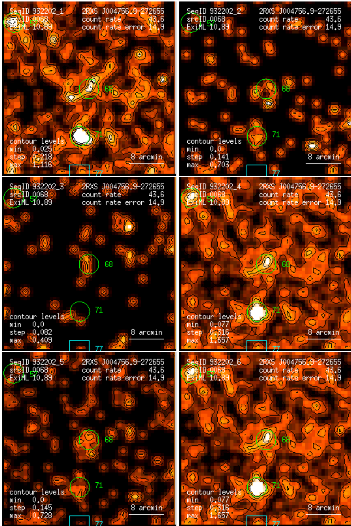
Figure 68: RASS 932202: detection 0068: band rate images, Gaussian filter: (1) PSPC channels 11 – 41, (2) 52 – 90, (3) 91 – 201, (4) 11 – 235, (5) 52 – 201, (6) 11 – 201. Broad band rates in counts/ks. Band rate contour levels in counts/ks/arcmin 2 .
