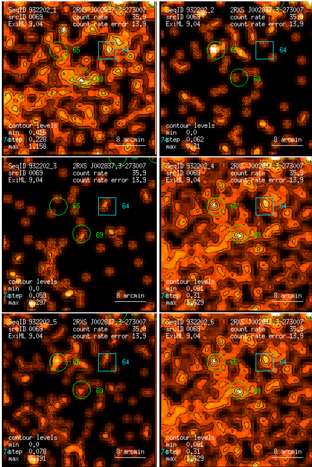
Figure 69: RASS 932202: detection 0069: band rate images, Gaussian filter: (1) PSPC channels 11 – 41, (2) 52 – 90, (3) 91 – 201, (4) 11 – 235, (5) 52 – 201, (6) 11 – 201. Broad band rates in counts/ks. Band rate contour levels in counts/ks/arcmin 2 .
