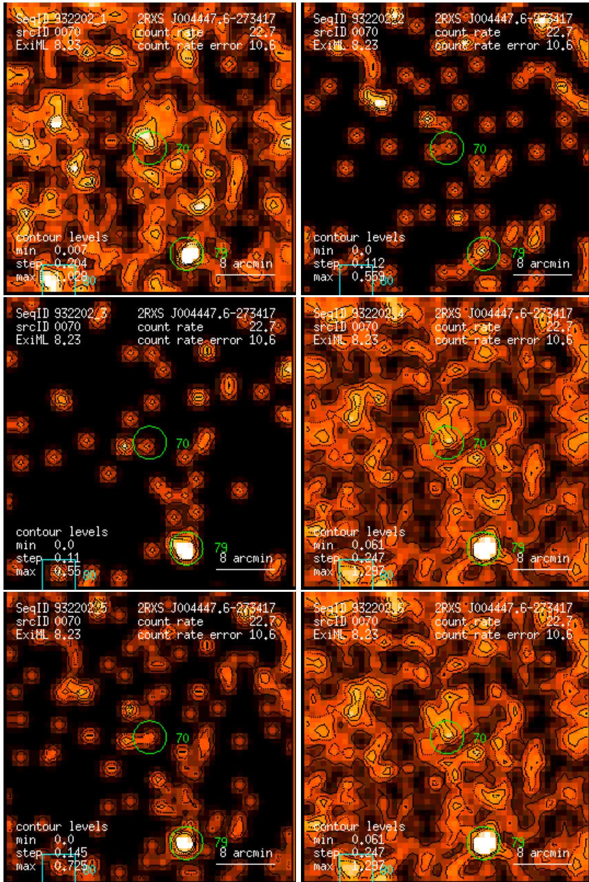
Figure 70: RASS 932202: detection 0070: band rate images, Gaussian filter: (1) PSPC channels 11 – 41, (2) 52 – 90, (3) 91 – 201, (4) 11 – 235, (5) 52 – 201, (6) 11 – 201. Broad band rates in counts/ks. Band rate contour levels in counts/ks/arcmin 2 .
