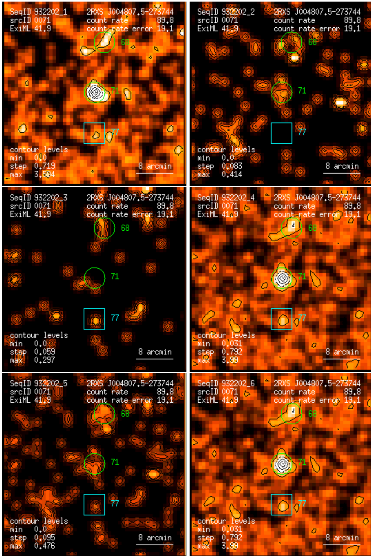
Figure 71: RASS 932202: detection 0071: band rate images, Gaussian filter: (1) PSPC channels 11 – 41, (2) 52 – 90, (3) 91 – 201, (4) 11 – 235, (5) 52 – 201, (6) 11 – 201. Broad band rates in counts/ks. Band rate contour levels in counts/ks/arcmin 2 .
