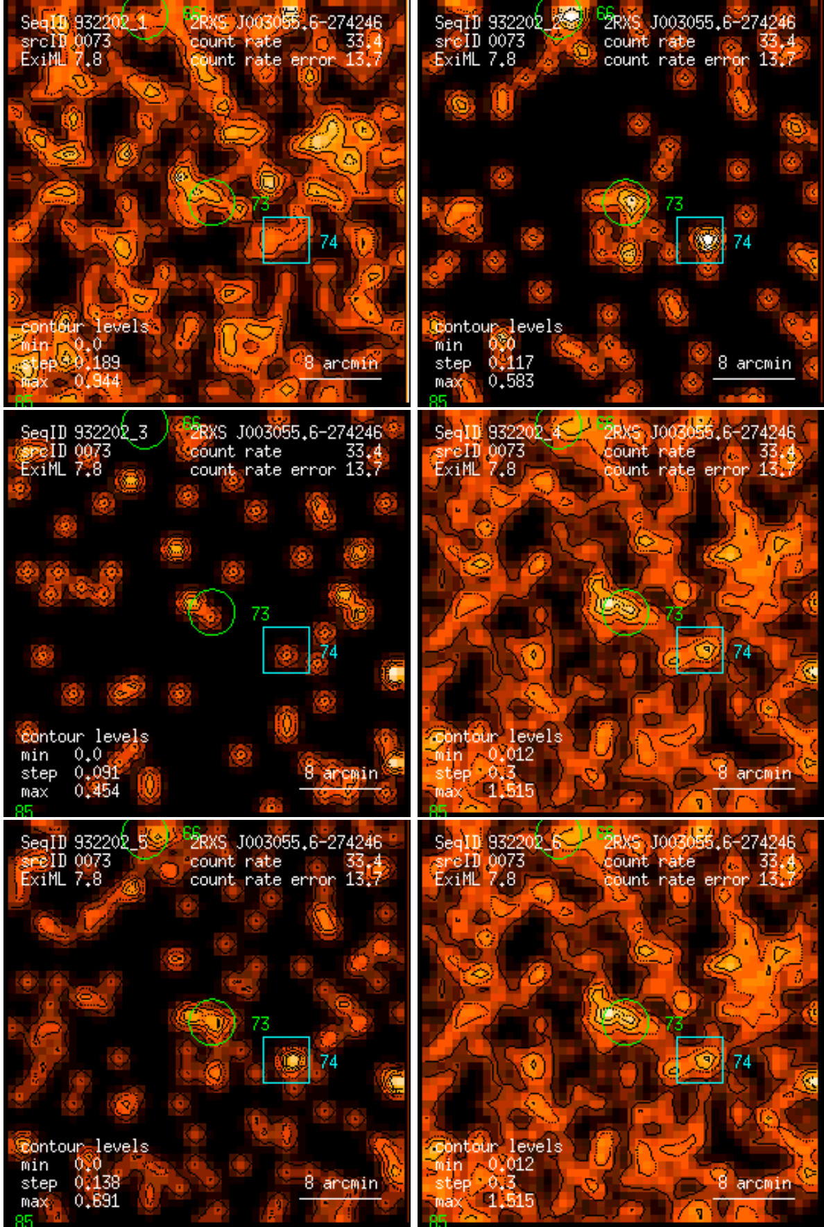
Figure 73: RASS 932202: detection 0073: band rate images, Gaussian filter: (1) PSPC channels 11 – 41, (2) 52 – 90, (3) 91 – 201, (4) 11 – 235, (5) 52 – 201, (6) 11 – 201. Broad band rates in counts/ks. Band rate contour levels in counts/ks/arcmin 2 .
