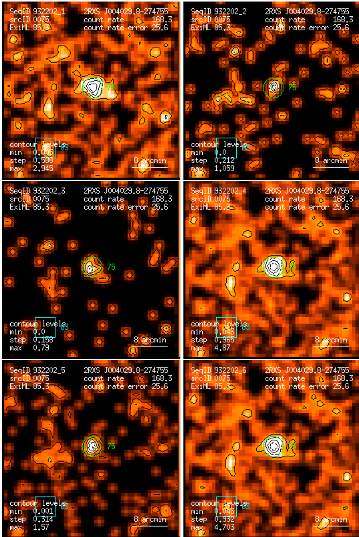
Figure 75: RASS 932202: detection 0075: band rate images, Gaussian filter: (1) PSPC channels 11 – 41, (2) 52 – 90, (3) 91 – 201, (4) 11 – 235, (5) 52 – 201, (6) 11 – 201. Broad band rates in counts/ks. Band rate contour levels in counts/ks/arcmin 2 .
