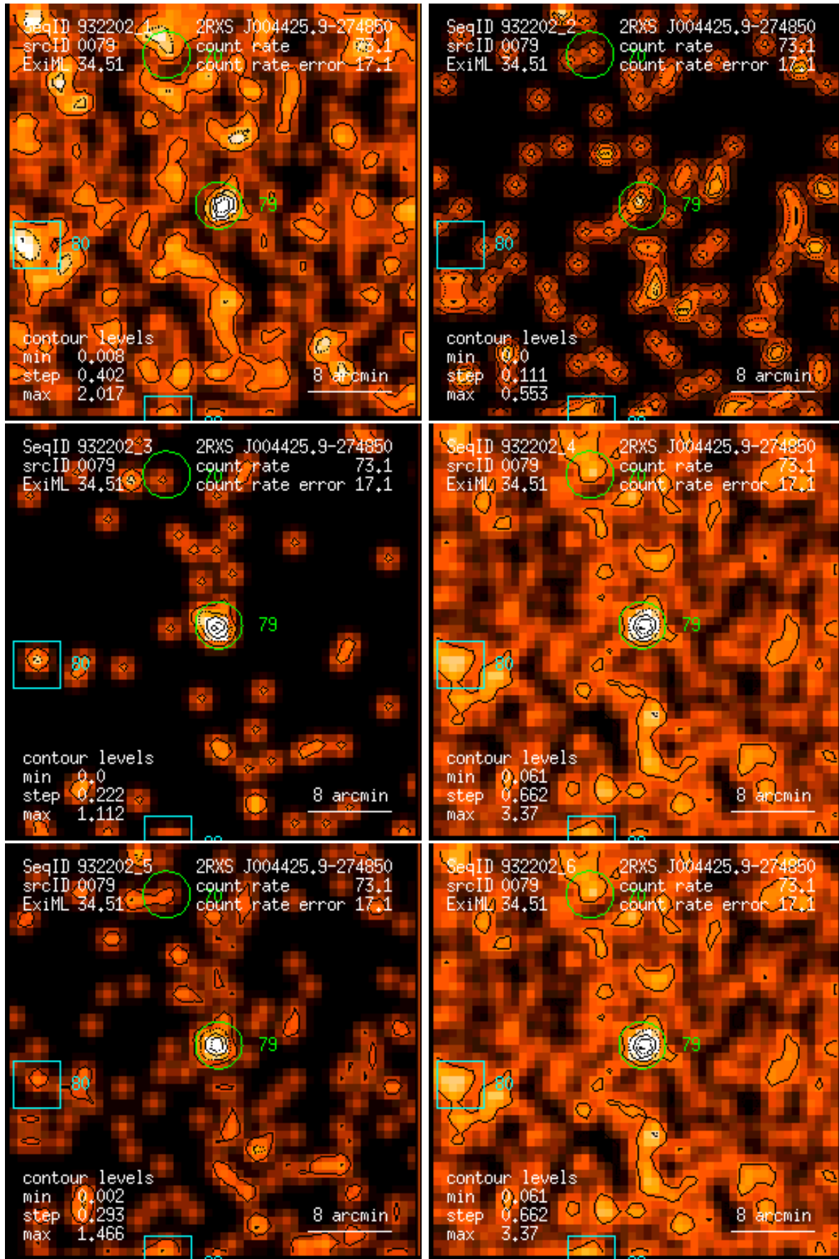
Figure 79: RASS 932202: detection 0079: band rate images, Gaussian filter: (1) PSPC channels 11 – 41, (2) 52 – 90, (3) 91 – 201, (4) 11 – 235, (5) 52 – 201, (6) 11 – 201. Broad band rates in counts/ks. Band rate contour levels in counts/ks/arcmin 2 .
