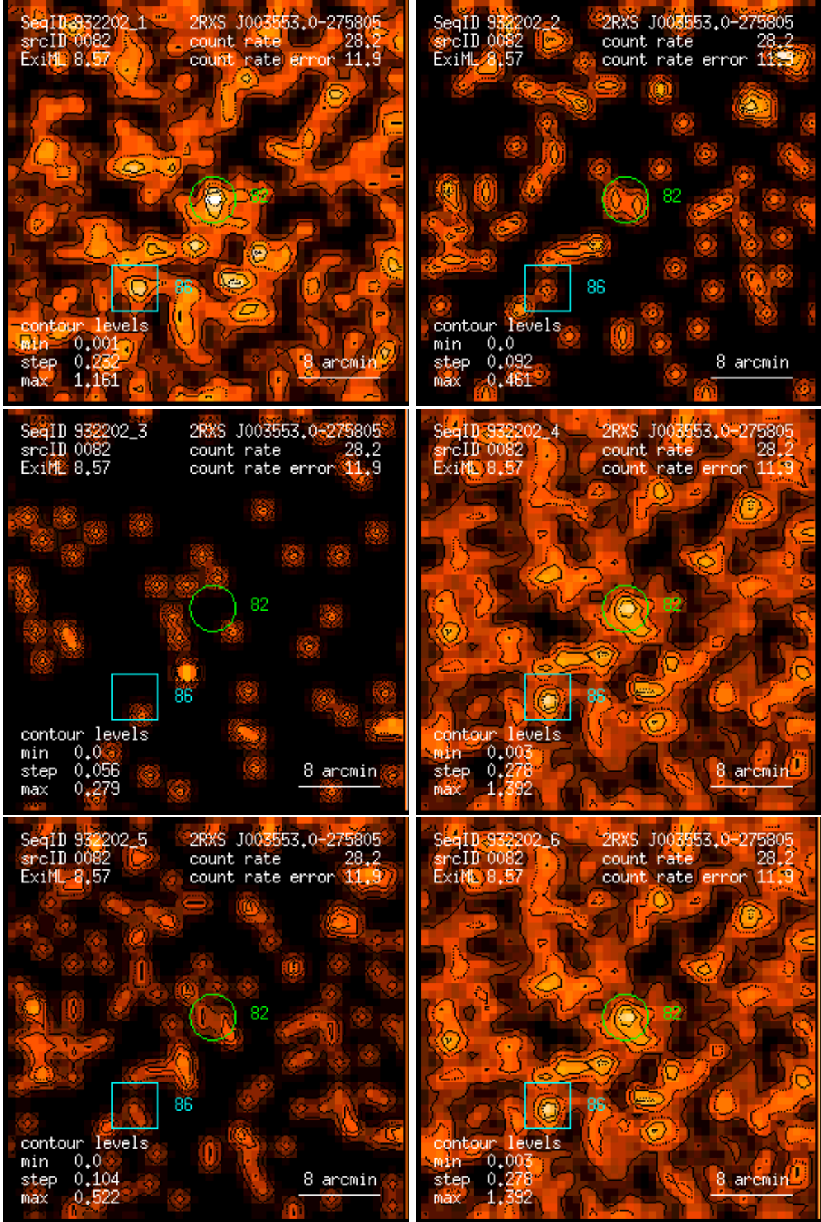
Figure 82: RASS 932202: detection 0082: band rate images, Gaussian filter: (1) PSPC channels 11 – 41, (2) 52 – 90, (3) 91 – 201, (4) 11 – 235, (5) 52 – 201, (6) 11 – 201. Broad band rates in counts/ks. Band rate contour levels in counts/ks/arcmin 2 .
