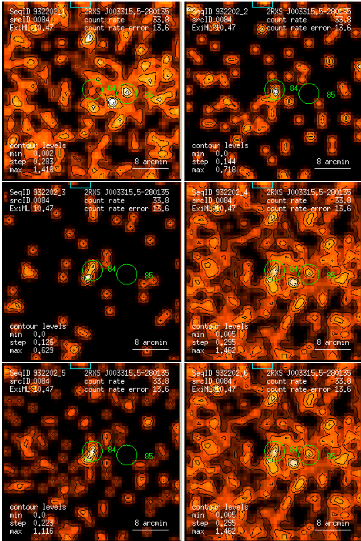
Figure 84: RASS 932202: detection 0084: band rate images, Gaussian filter: (1) PSPC channels 11 – 41, (2) 52 – 90, (3) 91 – 201, (4) 11 – 235, (5) 52 – 201, (6) 11 – 201. Broad band rates in counts/ks. Band rate contour levels in counts/ks/arcmin 2 .
