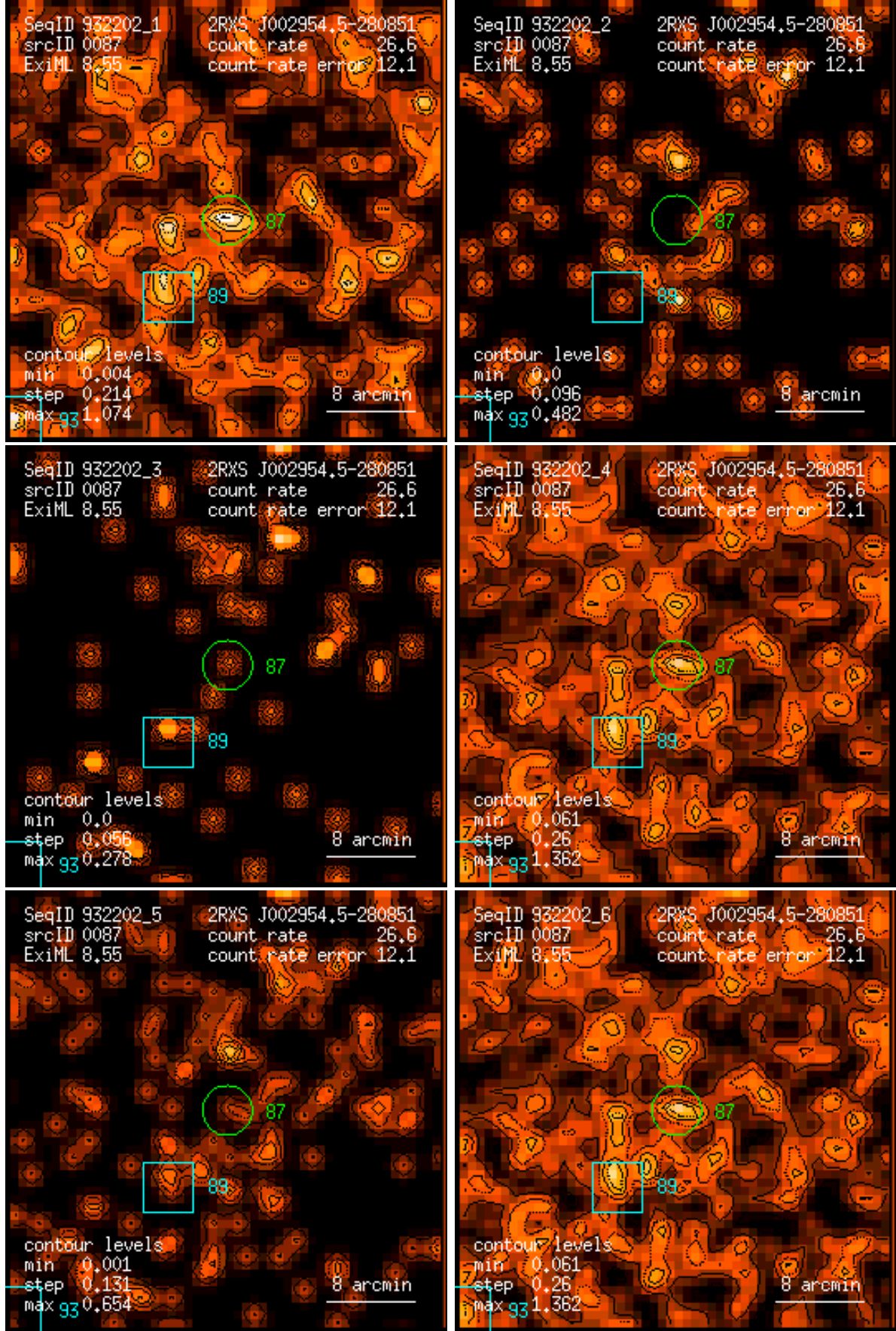
Figure 87: RASS 932202: detection 0087: band rate images, Gaussian filter: (1) PSPC channels 11 – 41, (2) 52 – 90, (3) 91 – 201, (4) 11 – 235, (5) 52 – 201, (6) 11 – 201. Broad band rates in counts/ks. Band rate contour levels in counts/ks/arcmin 2 .
