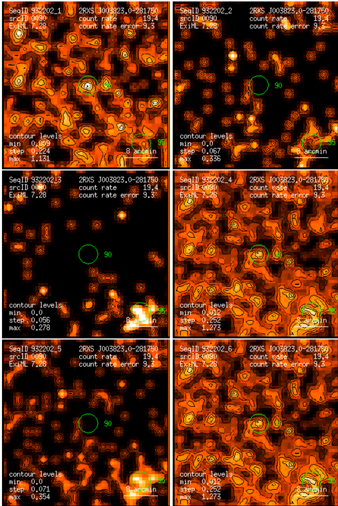
Figure 90: RASS 932202: detection 0090: band rate images, Gaussian filter: (1) PSPC channels 11 – 41, (2) 52 – 90, (3) 91 – 201, (4) 11 – 235, (5) 52 – 201, (6) 11 – 201. Broad band rates in counts/ks. Band rate contour levels in counts/ks/arcmin 2 .
