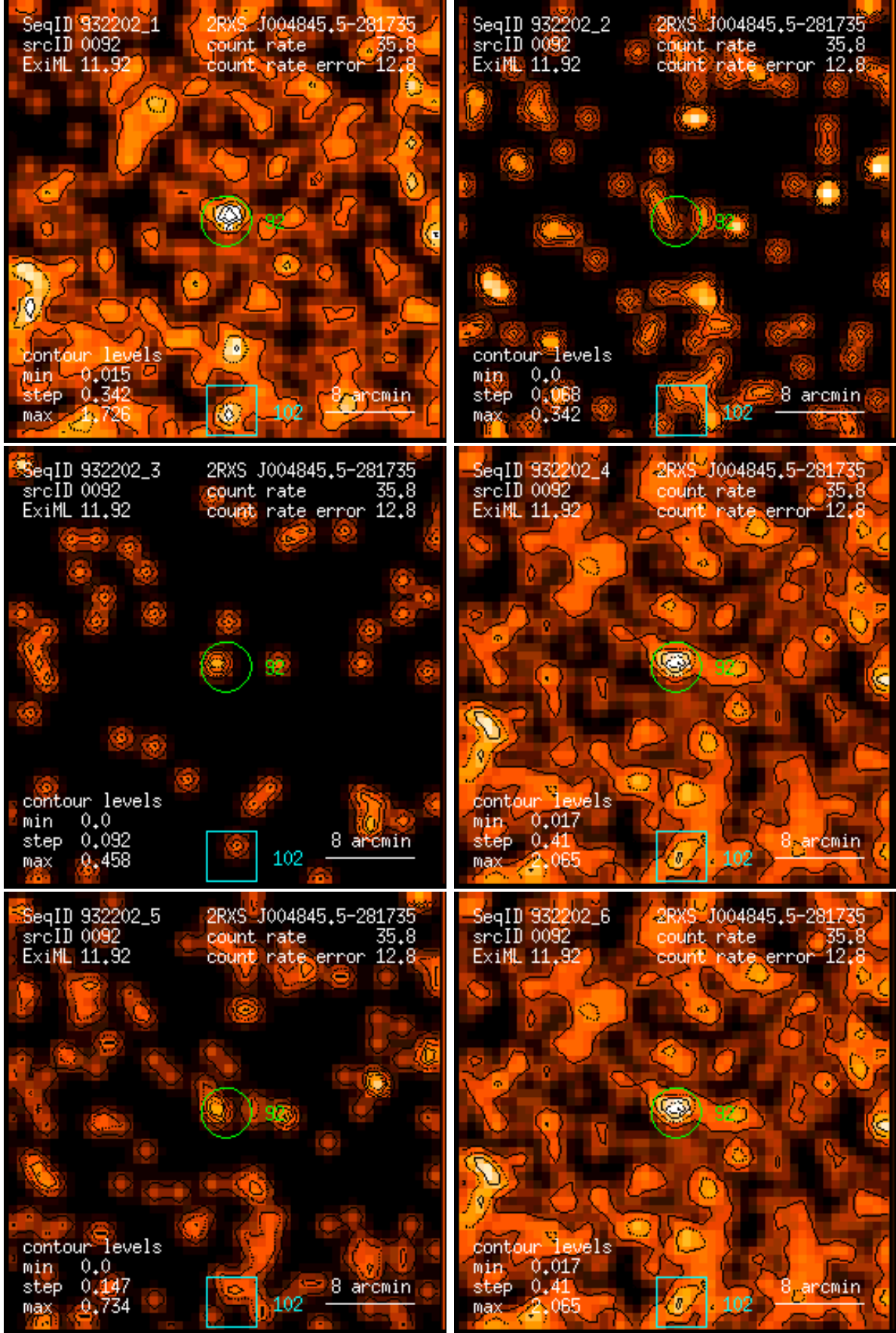
Figure 92: RASS 932202: detection 0092: band rate images, Gaussian filter: (1) PSPC channels 11 – 41, (2) 52 – 90, (3) 91 – 201, (4) 11 – 235, (5) 52 – 201, (6) 11 – 201. Broad band rates in counts/ks. Band rate contour levels in counts/ks/arcmin 2 .
