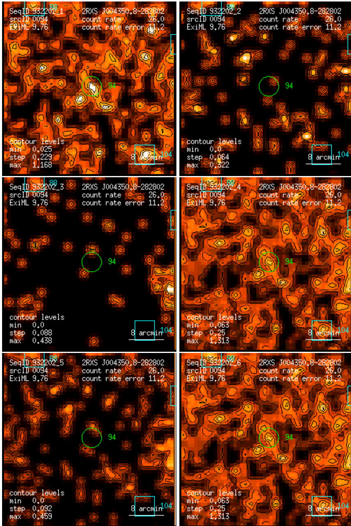
Figure 94: RASS 932202: detection 0094: band rate images, Gaussian filter: (1) PSPC channels 11 – 41, (2) 52 – 90, (3) 91 – 201, (4) 11 – 235, (5) 52 – 201, (6) 11 – 201. Broad band rates in counts/ks. Band rate contour levels in counts/ks/arcmin 2 .
