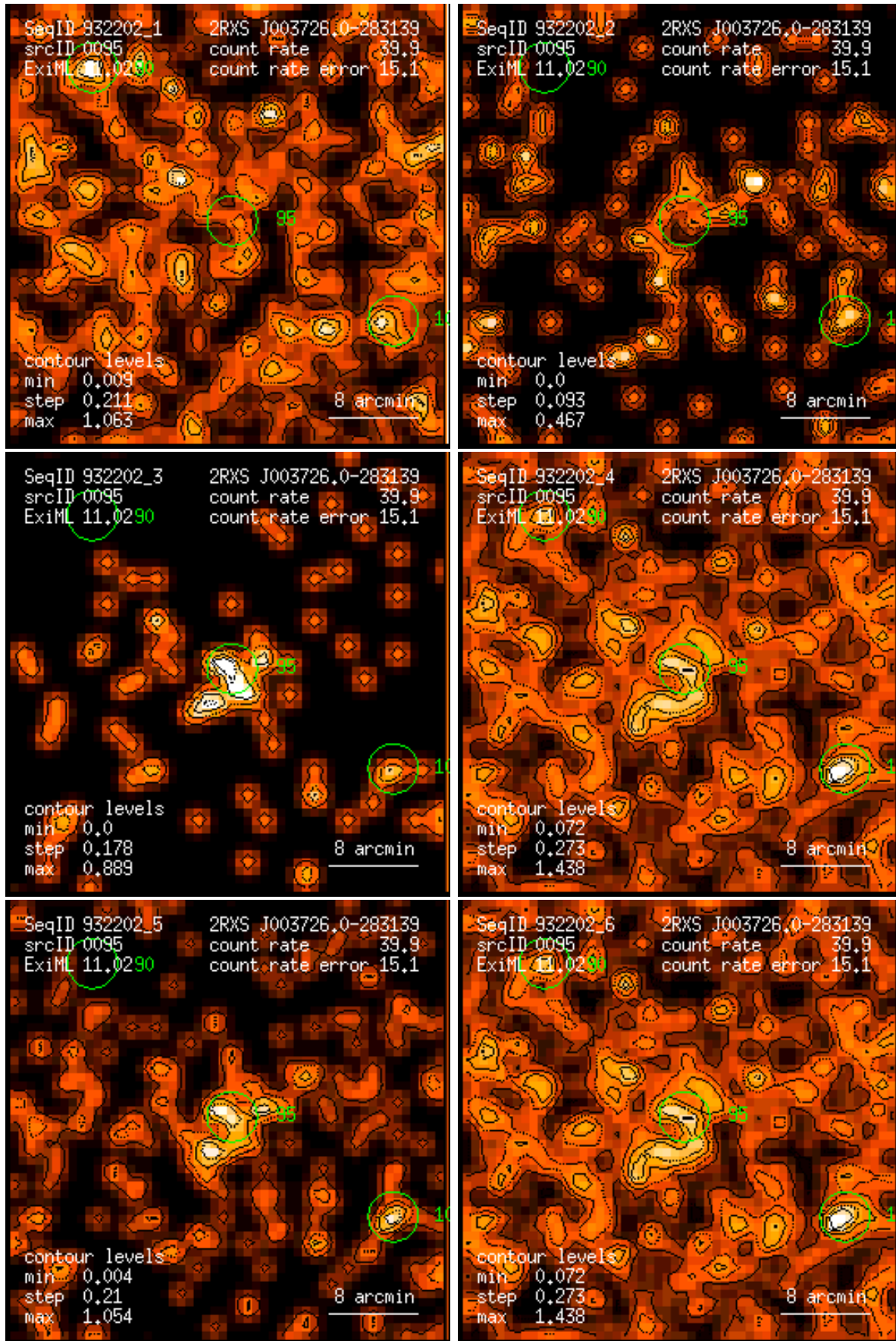
Figure 95: RASS 932202: detection 0095: band rate images, Gaussian filter: (1) PSPC channels 11 – 41, (2) 52 – 90, (3) 91 – 201, (4) 11 – 235, (5) 52 – 201, (6) 11 – 201. Broad band rates in counts/ks. Band rate contour levels in counts/ks/arcmin 2 .
