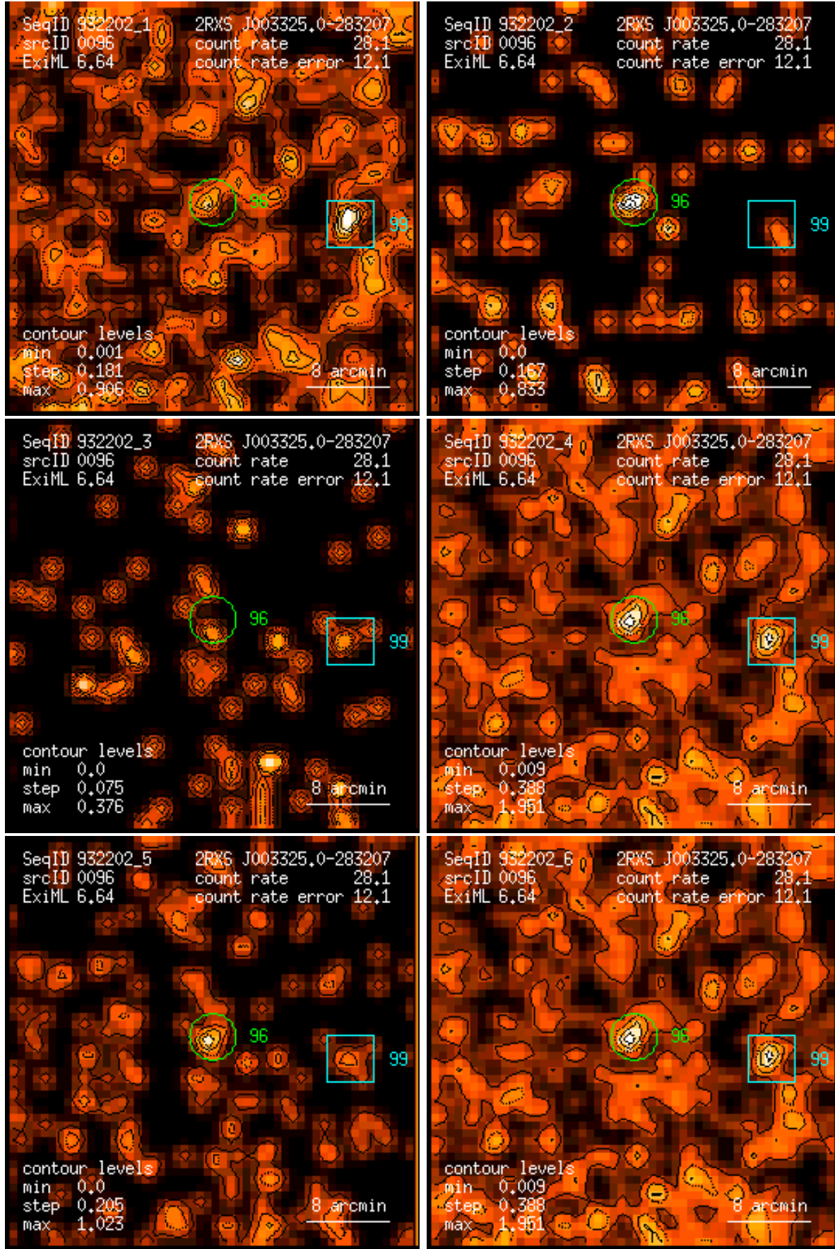
Figure 96: RASS 932202: detection 0096: band rate images, Gaussian filter: (1) PSPC channels 11 – 41, (2) 52 – 90, (3) 91 – 201, (4) 11 – 235, (5) 52 – 201, (6) 11 – 201. Broad band rates in counts/ks. Band rate contour levels in counts/ks/arcmin 2 .
