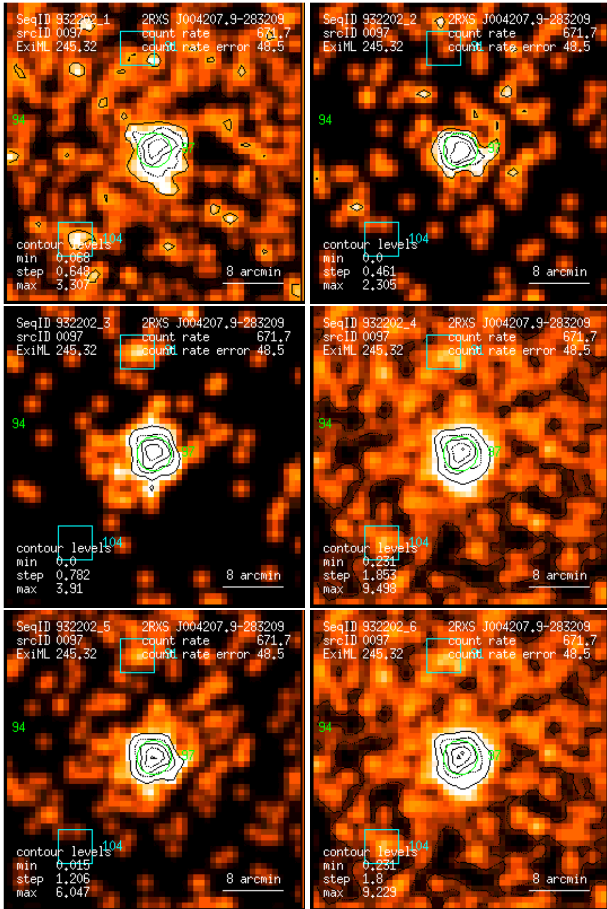
Figure 97: RASS 932202: detection 0097: band rate images, Gaussian filter: (1) PSPC channels 11 – 41, (2) 52 – 90, (3) 91 – 201, (4) 11 – 235, (5) 52 – 201, (6) 11 – 201. Broad band rates in counts/ks. Band rate contour levels in counts/ks/arcmin 2 .
