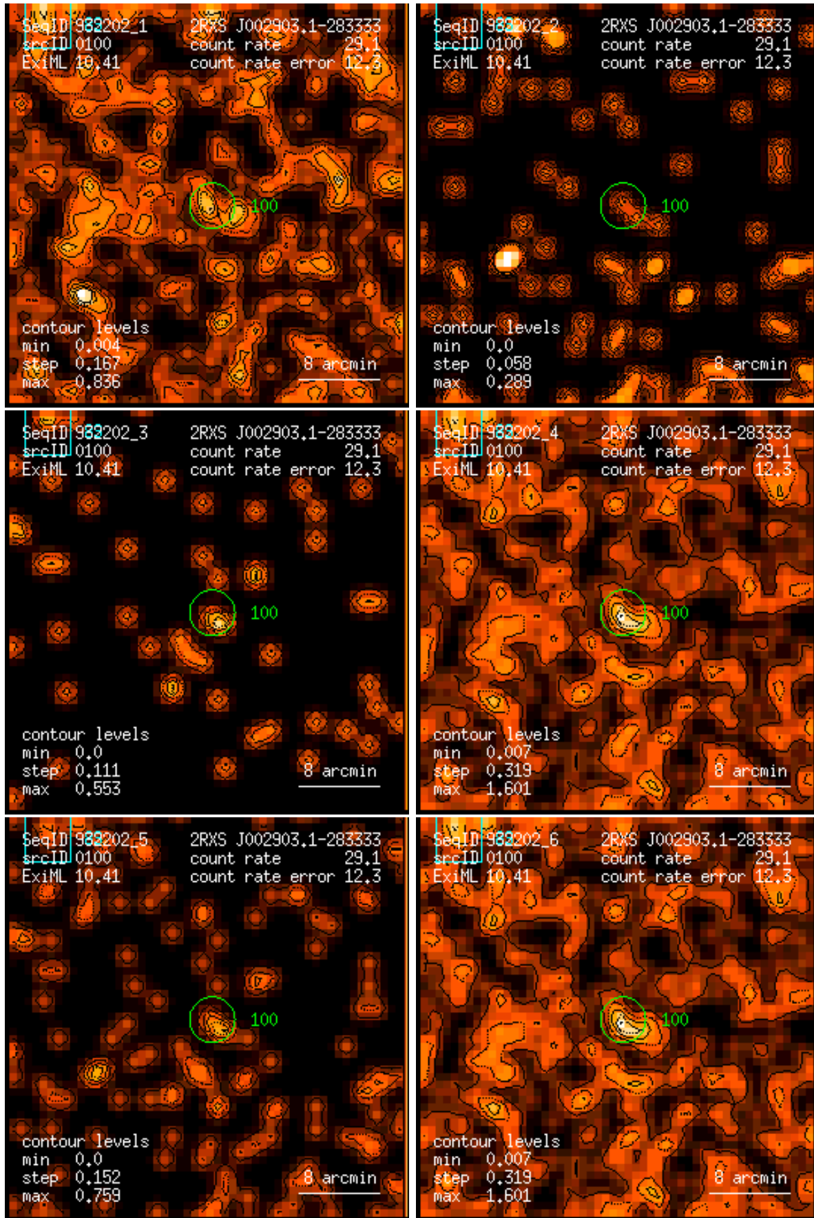
Figure 100: RASS 932202: detection 0100: band rate images, Gaussian filter: (1) PSPC channels 11 – 41, (2) 52 – 90, (3) 91 – 201, (4) 11 – 235, (5) 52 – 201, (6) 11 – 201. Broad band rates in counts/ks. Band rate contour levels in counts/ks/arcmin 2 .
