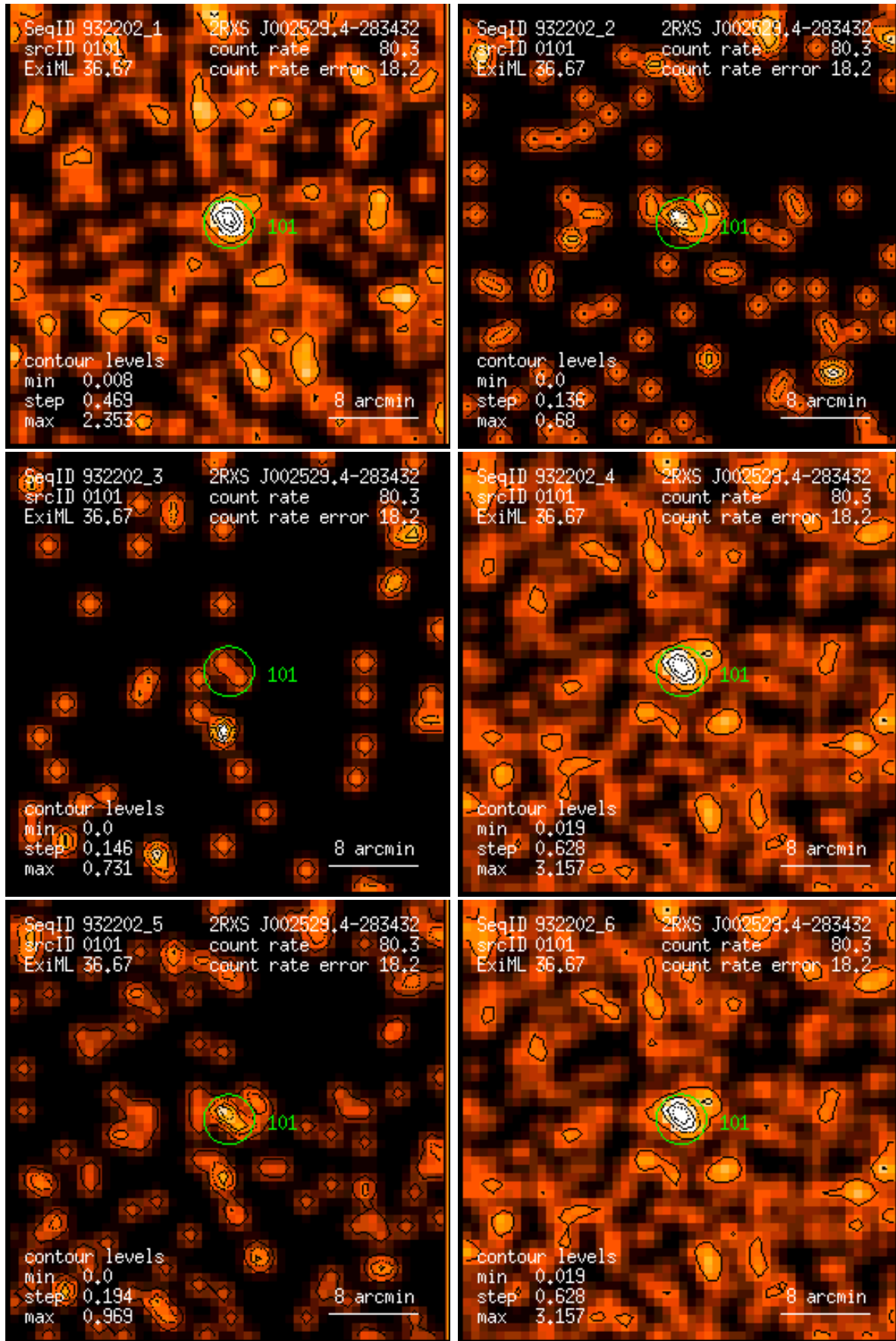
Figure 101: RASS 932202: detection 0101: band rate images, Gaussian filter: (1) PSPC channels 11 – 41, (2) 52 – 90, (3) 91 – 201, (4) 11 – 235, (5) 52 – 201, (6) 11 – 201. Broad band rates in counts/ks. Band rate contour levels in counts/ks/arcmin 2 .
