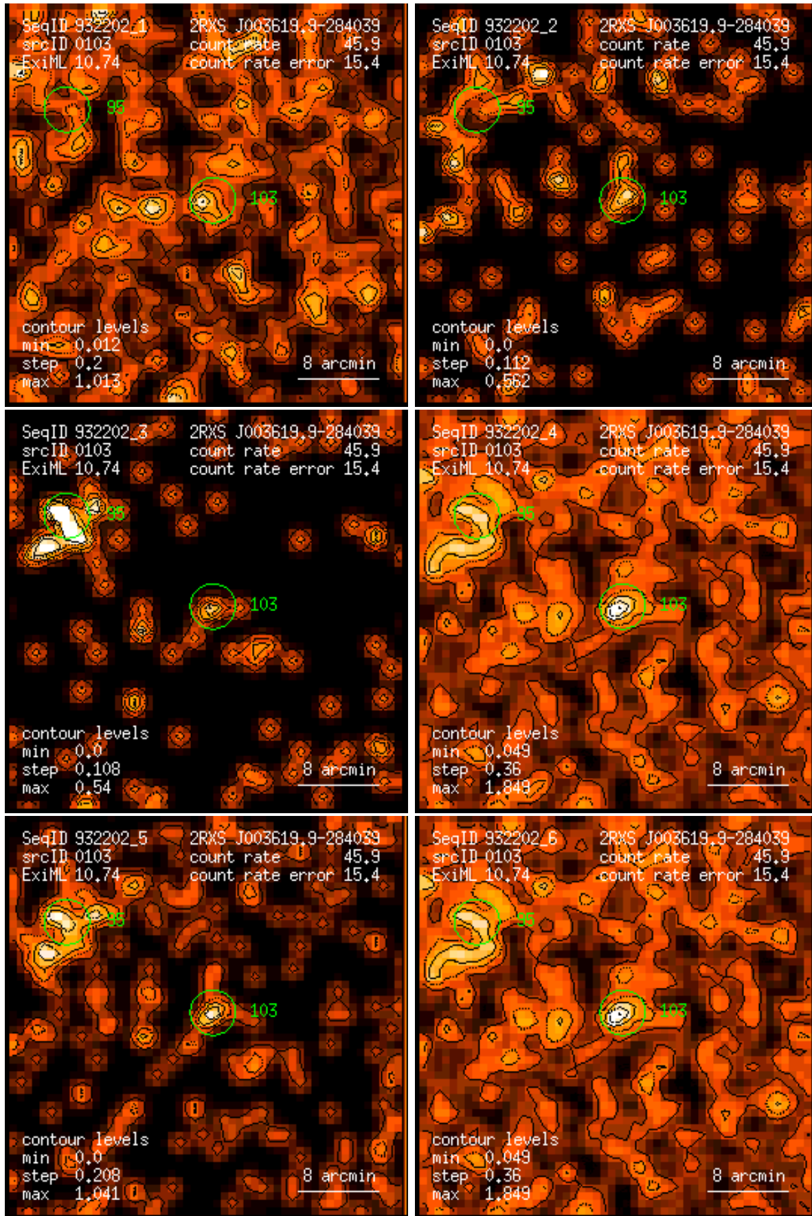
Figure 103: RASS 932202: detection 0103: band rate images, Gaussian filter: (1) PSPC channels 11 – 41, (2) 52 – 90, (3) 91 – 201, (4) 11 – 235, (5) 52 – 201, (6) 11 – 201. Broad band rates in counts/ks. Band rate contour levels in counts/ks/arcmin 2 .
