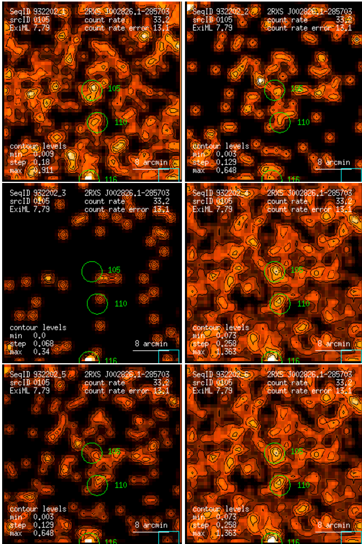
Figure 105: RASS 932202: detection 0105: band rate images, Gaussian filter: (1) PSPC channels 11 – 41, (2) 52 – 90, (3) 91 – 201, (4) 11 – 235, (5) 52 – 201, (6) 11 – 201. Broad band rates in counts/ks. Band rate contour levels in counts/ks/arcmin 2 .
