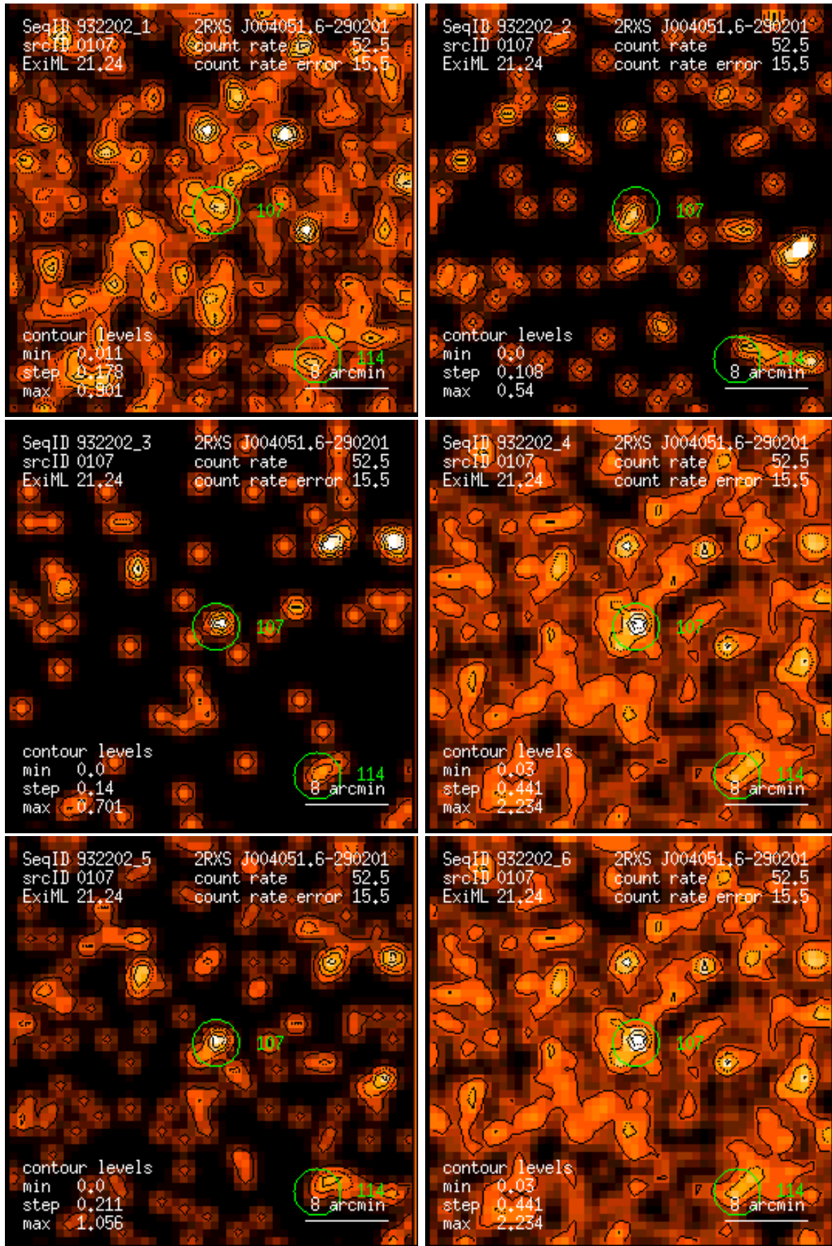
Figure 107: RASS 932202: detection 0107: band rate images, Gaussian filter: (1) PSPC channels 11 – 41, (2) 52 – 90, (3) 91 – 201, (4) 11 – 235, (5) 52 – 201, (6) 11 – 201. Broad band rates in counts/ks. Band rate contour levels in counts/ks/arcmin 2 .
