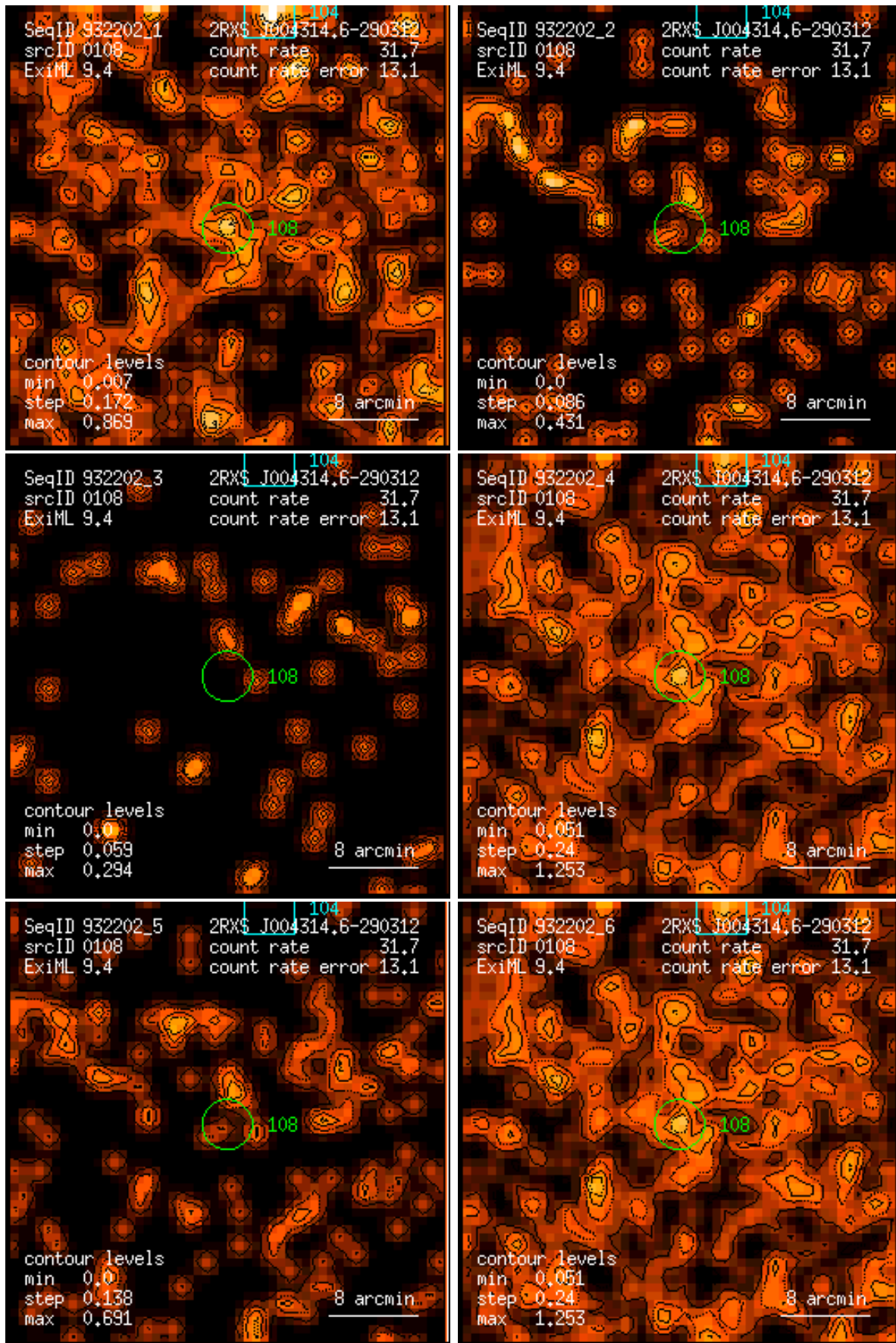
Figure 108: RASS 932202: detection 0108: band rate images, Gaussian filter: (1) PSPC channels 11 – 41, (2) 52 – 90, (3) 91 – 201, (4) 11 – 235, (5) 52 – 201, (6) 11 – 201. Broad band rates in counts/ks. Band rate contour levels in counts/ks/arcmin 2 .
