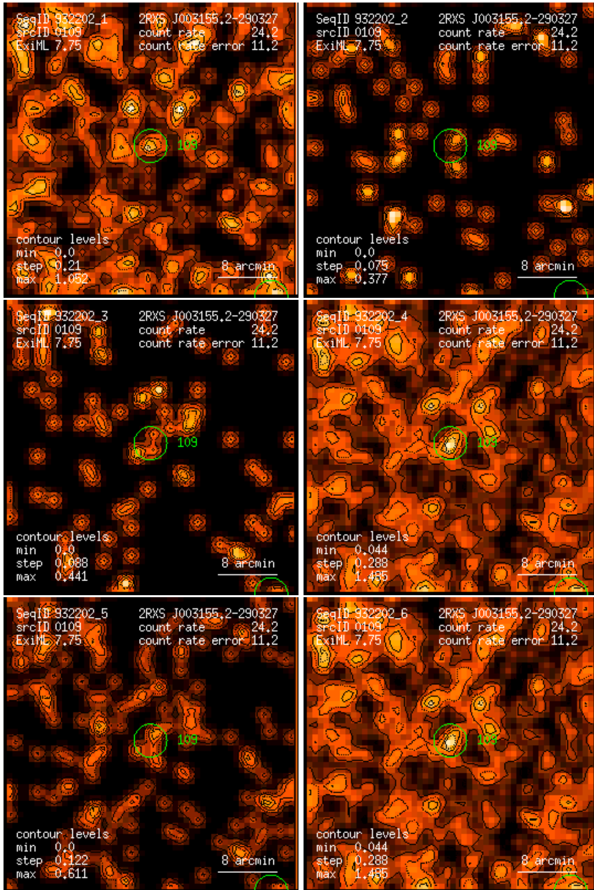
Figure 109: RASS 932202: detection 0109: band rate images, Gaussian filter: (1) PSPC channels 11 – 41, (2) 52 – 90, (3) 91 – 201, (4) 11 – 235, (5) 52 – 201, (6) 11 – 201. Broad band rates in counts/ks. Band rate contour levels in counts/ks/arcmin 2 .
