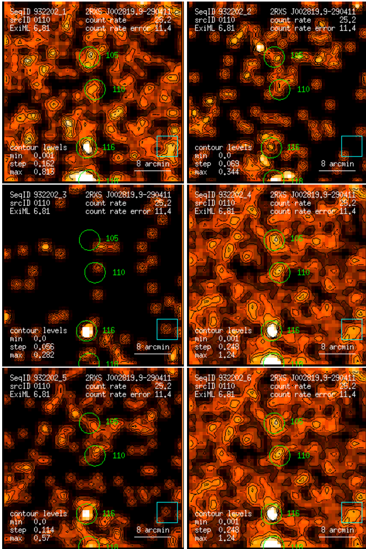
Figure 110: RASS 932202: detection 0110: band rate images, Gaussian filter: (1) PSPC channels 11 – 41, (2) 52 – 90, (3) 91 – 201, (4) 11 – 235, (5) 52 – 201, (6) 11 – 201. Broad band rates in counts/ks. Band rate contour levels in counts/ks/arcmin 2 .
