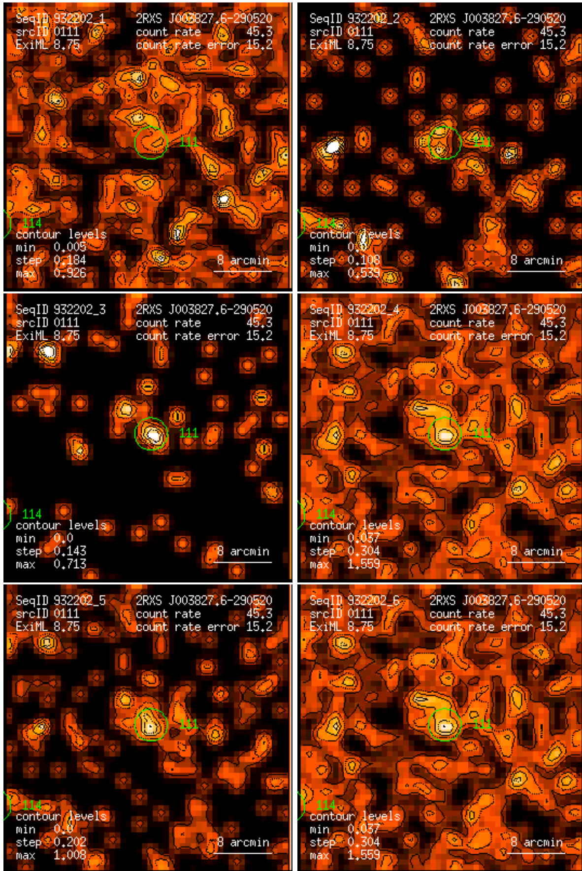
Figure 111: RASS 932202: detection 0111: band rate images, Gaussian filter: (1) PSPC channels 11 – 41, (2) 52 – 90, (3) 91 – 201, (4) 11 – 235, (5) 52 – 201, (6) 11 – 201. Broad band rates in counts/ks. Band rate contour levels in counts/ks/arcmin 2 .
