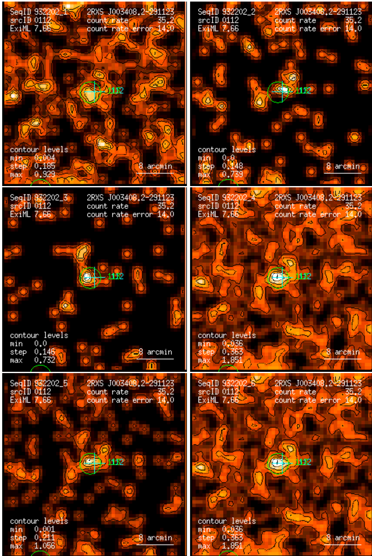
Figure 112: RASS 932202: detection 0112: band rate images, Gaussian filter: (1) PSPC channels 11 – 41, (2) 52 – 90, (3) 91 – 201, (4) 11 – 235, (5) 52 – 201, (6) 11 – 201. Broad band rates in counts/ks. Band rate contour levels in counts/ks/arcmin 2 .
