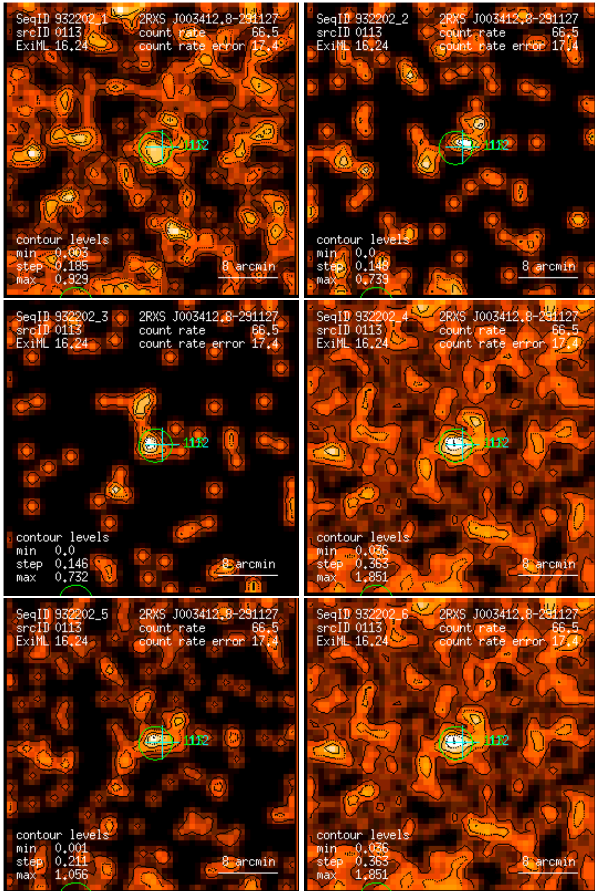
Figure 113: RASS 932202: detection 0113: band rate images, Gaussian filter: (1) PSPC channels 11 – 41, (2) 52 – 90, (3) 91 – 201, (4) 11 – 235, (5) 52 – 201, (6) 11 – 201. Broad band rates in counts/ks. Band rate contour levels in counts/ks/arcmin 2 .
