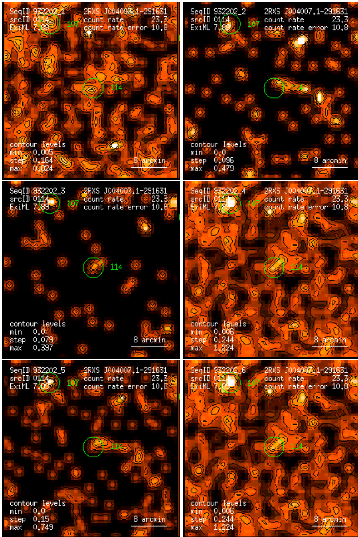
Figure 114: RASS 932202: detection 0114: band rate images, Gaussian filter: (1) PSPC channels 11 – 41, (2) 52 – 90, (3) 91 – 201, (4) 11 – 235, (5) 52 – 201, (6) 11 – 201. Broad band rates in counts/ks. Band rate contour levels in counts/ks/arcmin 2 .
