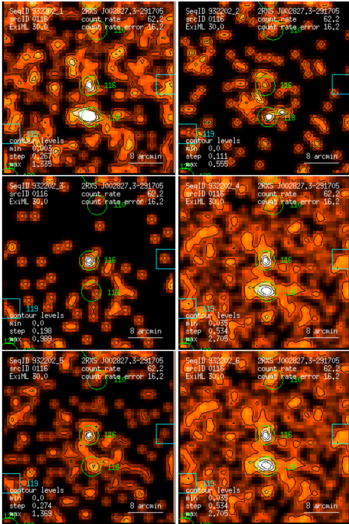
Figure 116: RASS 932202: detection 0116: band rate images, Gaussian filter: (1) PSPC channels 11 – 41, (2) 52 – 90, (3) 91 – 201, (4) 11 – 235, (5) 52 – 201, (6) 11 – 201. Broad band rates in counts/ks. Band rate contour levels in counts/ks/arcmin 2 .
