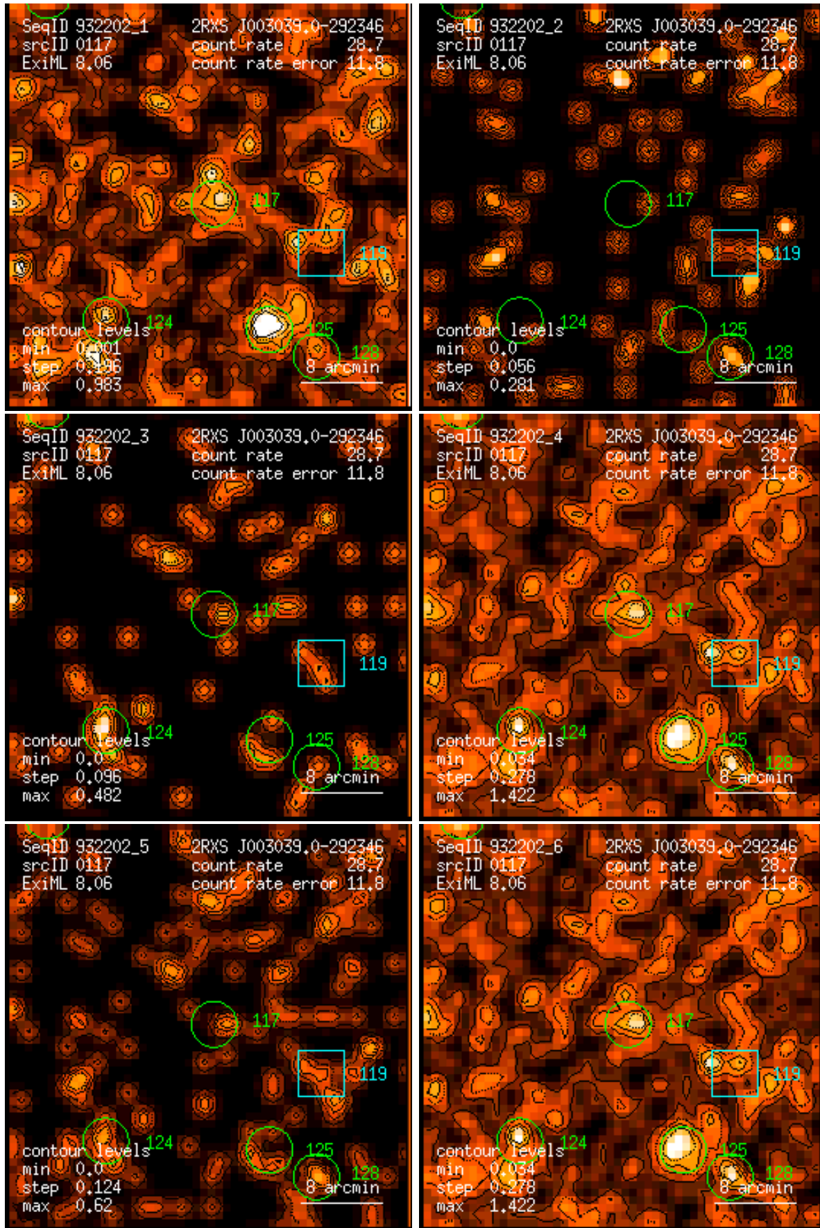
Figure 117: RASS 932202: detection 0117: band rate images, Gaussian filter: (1) PSPC channels 11 – 41, (2) 52 – 90, (3) 91 – 201, (4) 11 – 235, (5) 52 – 201, (6) 11 – 201. Broad band rates in counts/ks. Band rate contour levels in counts/ks/arcmin 2 .
