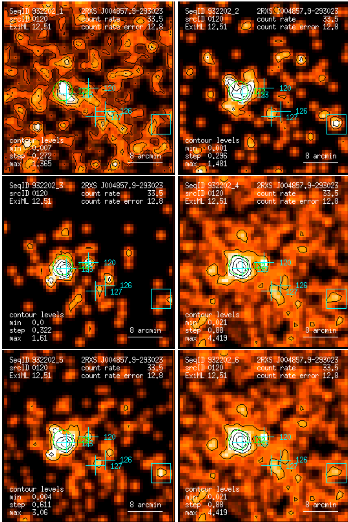
Figure 120: RASS 932202: detection 0120: band rate images, Gaussian filter: (1) PSPC channels 11 – 41, (2) 52 – 90, (3) 91 – 201, (4) 11 – 235, (5) 52 – 201, (6) 11 – 201. Broad band rates in counts/ks. Band rate contour levels in counts/ks/arcmin 2 .
