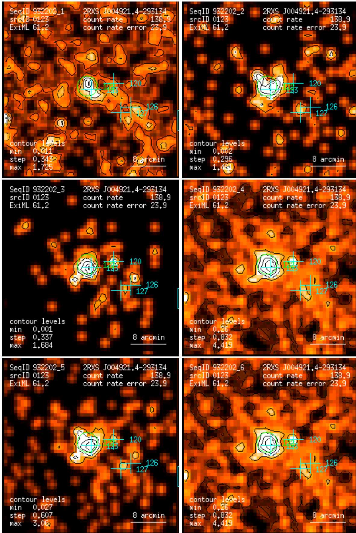
Figure 123: RASS 932202: detection 0123: band rate images, Gaussian filter: (1) PSPC channels 11 – 41, (2) 52 – 90, (3) 91 – 201, (4) 11 – 235, (5) 52 – 201, (6) 11 – 201. Broad band rates in counts/ks. Band rate contour levels in counts/ks/arcmin 2 .
