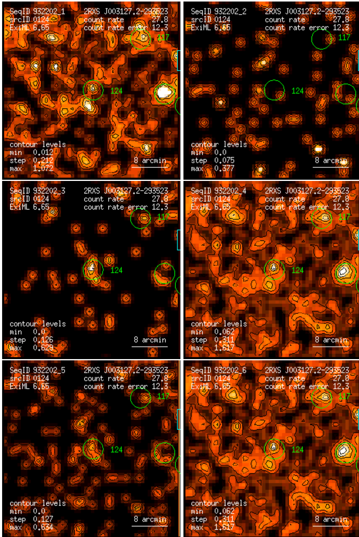
Figure 124: RASS 932202: detection 0124: band rate images, Gaussian filter: (1) PSPC channels 11 – 41, (2) 52 – 90, (3) 91 – 201, (4) 11 – 235, (5) 52 – 201, (6) 11 – 201. Broad band rates in counts/ks. Band rate contour levels in counts/ks/arcmin 2 .
