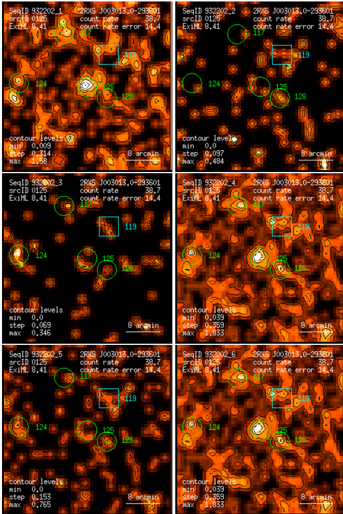
Figure 125: RASS 932202: detection 0125: band rate images, Gaussian filter: (1) PSPC channels 11 – 41, (2) 52 – 90, (3) 91 – 201, (4) 11 – 235, (5) 52 – 201, (6) 11 – 201. Broad band rates in counts/ks. Band rate contour levels in counts/ks/arcmin 2 .
