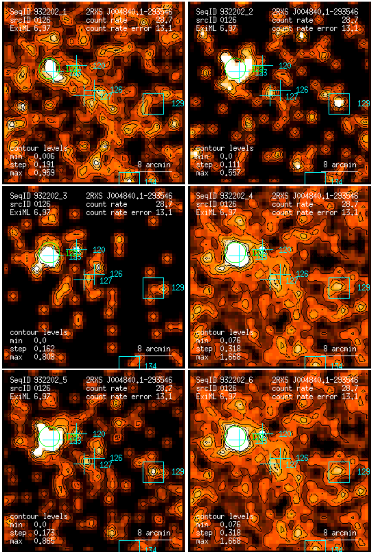
Figure 126: RASS 932202: detection 0126: band rate images, Gaussian filter: (1) PSPC channels 11 – 41, (2) 52 – 90, (3) 91 – 201, (4) 11 – 235, (5) 52 – 201, (6) 11 – 201. Broad band rates in counts/ks. Band rate contour levels in counts/ks/arcmin 2 .
